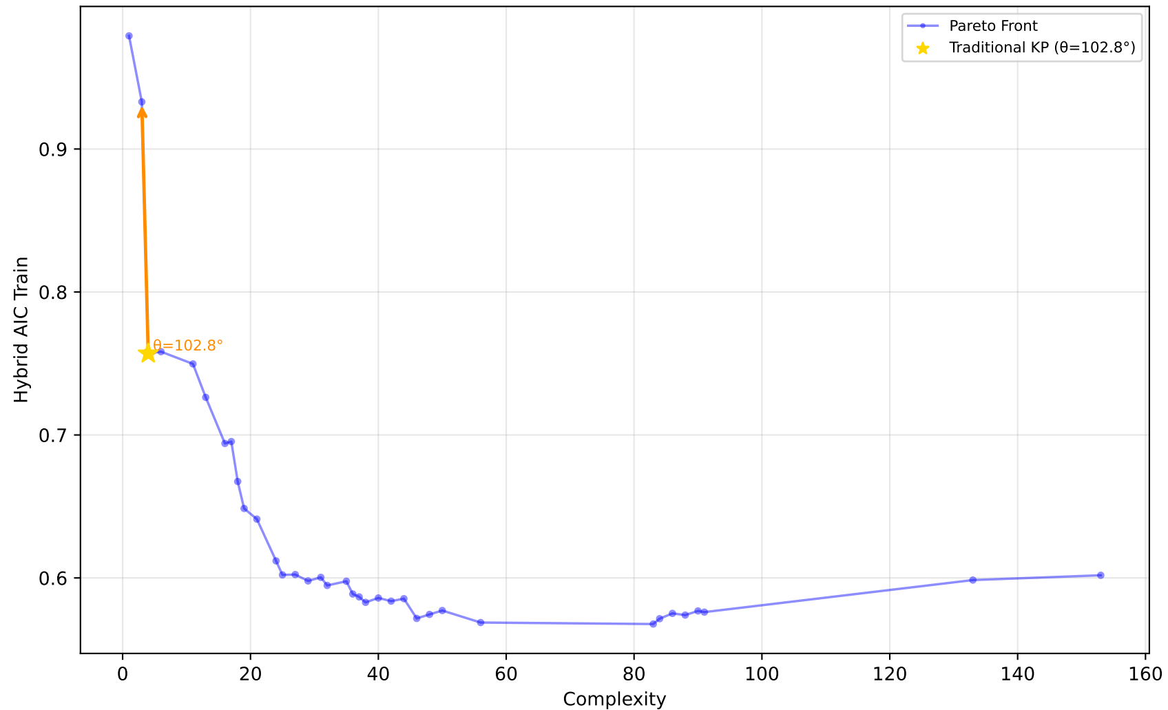
605_fri_c2_250_25 - Run 9 - MVP - Hybrid AIC Train \lambda_1=0.10, \lambda_2=0.00, \lambda_3=0.00 | Difficulty: 1.00 | Method: hmr
