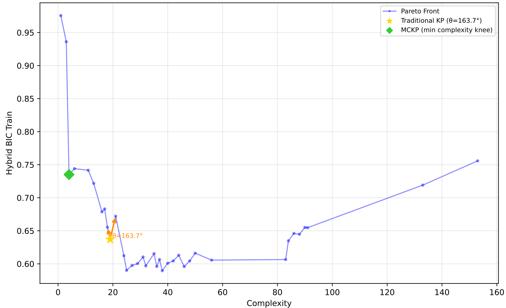
605_fri_c2_250_25 - Run 9 - MVP - Hybrid BIC Train \lambda_1=0.30, \lambda_2=0.00, \lambda_3=1.00 | Difficulty: 1.00 | Method: hmr
