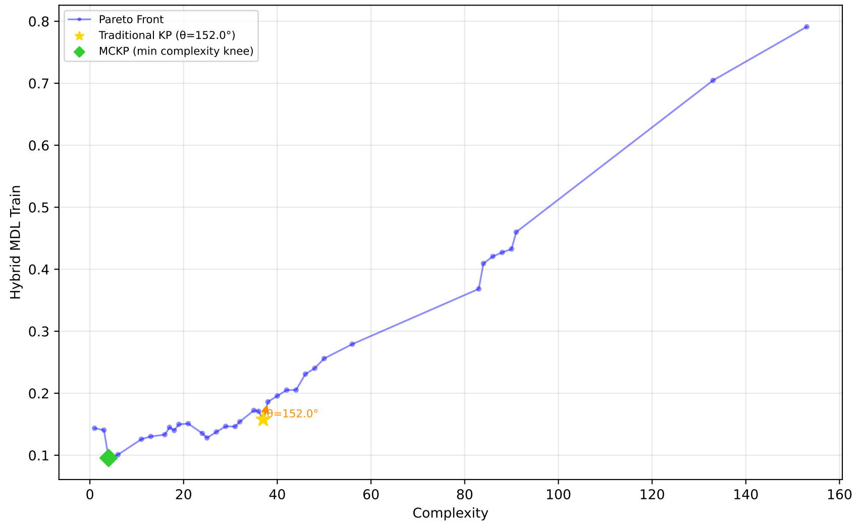
605_fri_c2_250_25 - Run 9 - SVP - Hybrid MDL Train \lambda_1=0.10, \lambda_2=0.00, \lambda_3=0.00 | Difficulty: 1.00 | Method: hmr
