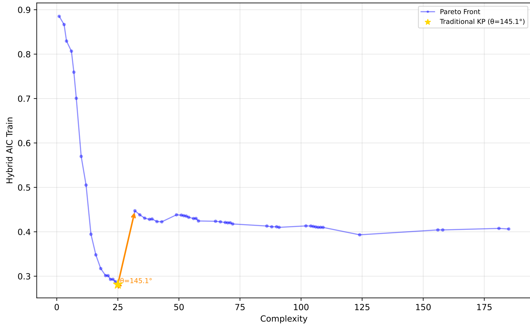
227_cpu_small - Run 10 - MVP - Hybrid AIC Train \lambda_1=0.00, \bar{\lambda}_2=0.90, \lambda_3=0.10 | Difficulty: 1.00 | Method: hmr
