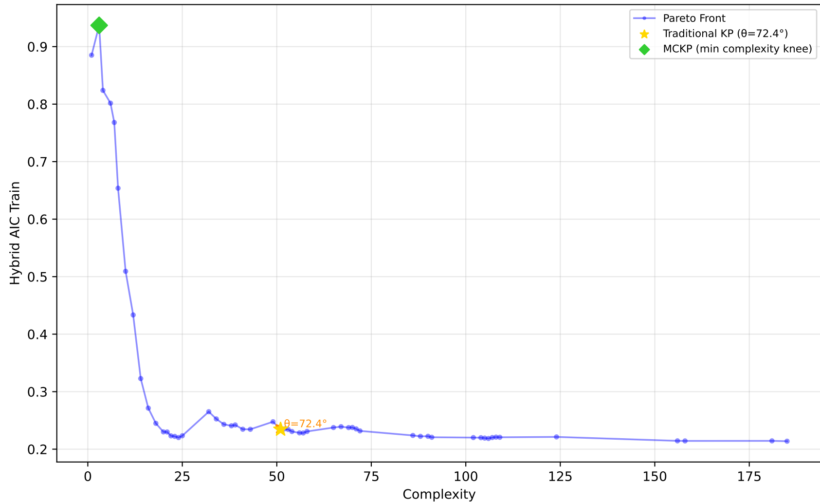
227_cpu_small - Run 10 - MVP - Hybrid AIC Train \lambda_1=0.80, \bar{\lambda}_2=0.20, \lambda_3=0.00 | Difficulty: 1.00 | Method: hmr
