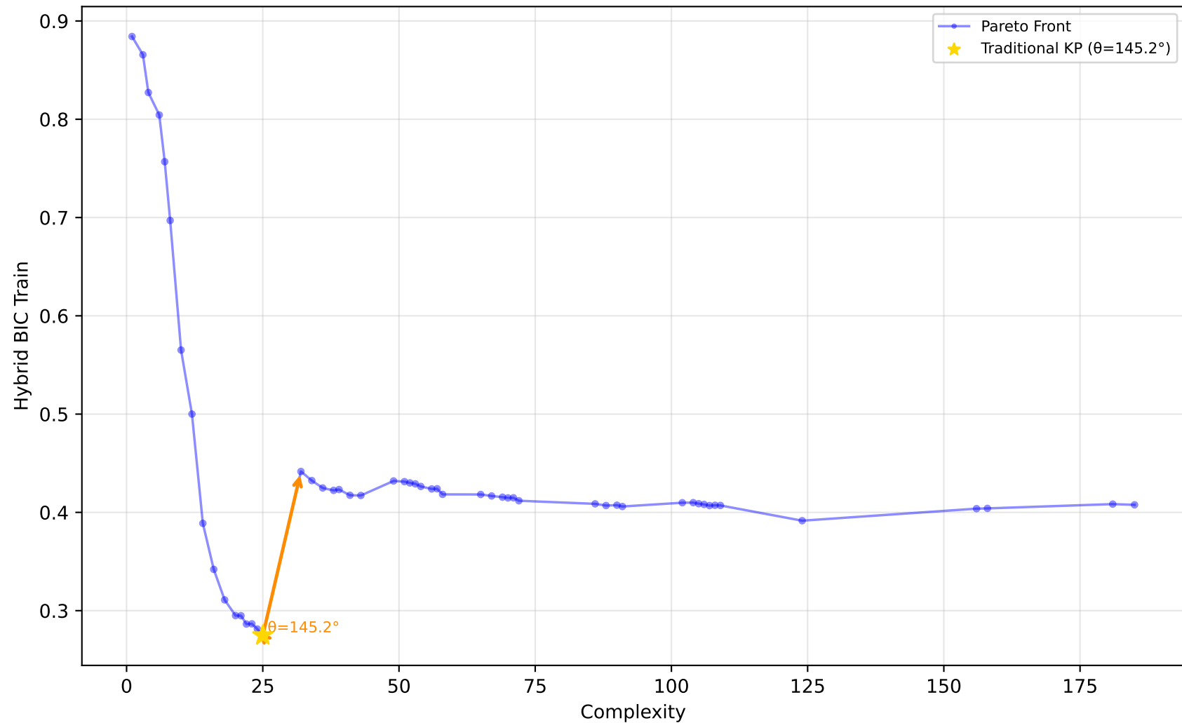
227_cpu_small - Run 10 - MVP - Hybrid BIC Train \lambda_1=0.00, \lambda_2=0.90, \lambda_3=0.10 | Difficulty: 1.00 | Method: hmr
