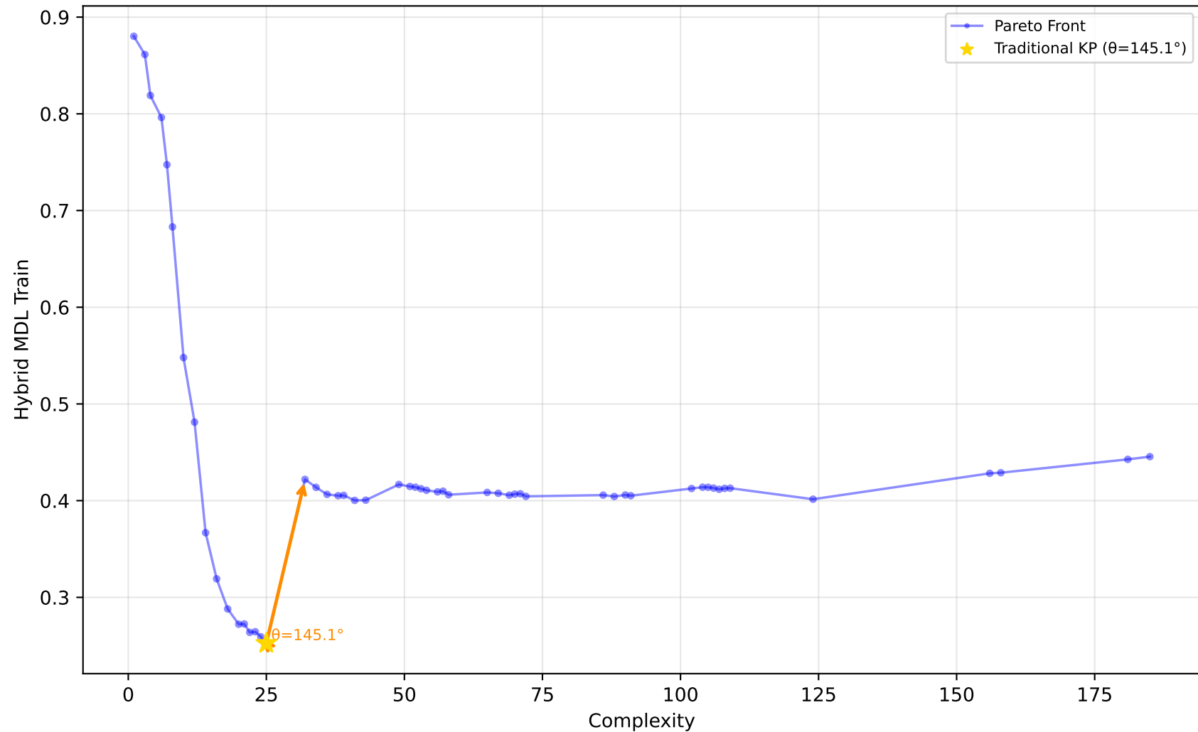
227_cpu_small - Run 10 - MVP - Hybrid MDL Train \lambda_1=0.00, \lambda_2=0.90, \lambda_3=0.10 | Difficulty: 1.00 | Method: hmr
