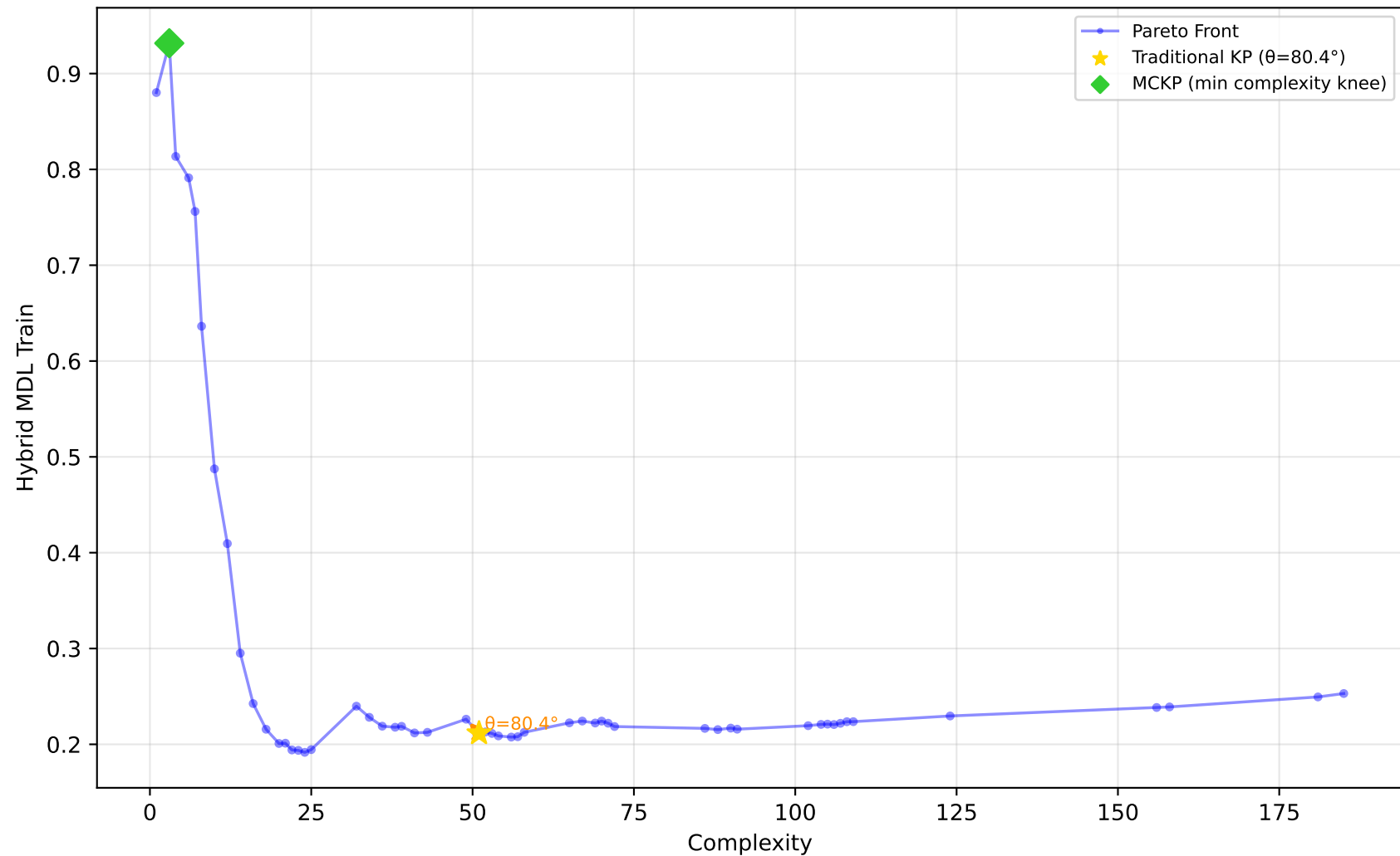
227_cpu_small - Run 10 - MVP - Hybrid MDL Train \lambda_1=0.80, \lambda_2=0.20, \lambda_3=0.00 | Difficulty: 1.00 | Method: hmr
