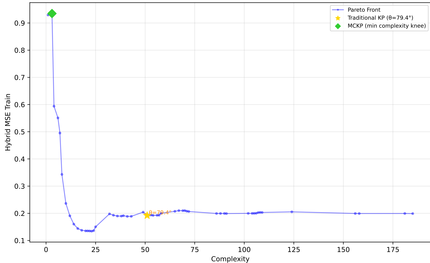
227_cpu_small - Run 10 - MVP - Hybrid MSE Train \lambda_1=0.80, \lambda_2=0.20, \lambda_3=0.00 | Difficulty: 1.00 | Method: hmr
