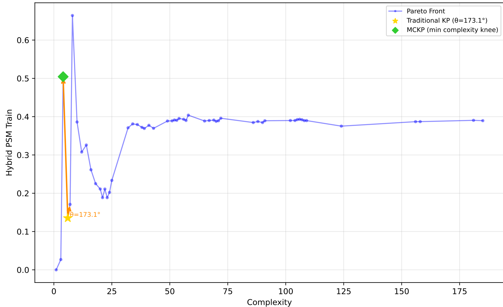
227_cpu_small - Run 10 - MVP - Hybrid PSM Train \lambda_1=0.00, \lambda_2=0.90, \lambda_3=0.10 | Difficulty: 1.00 | Method: hmr
