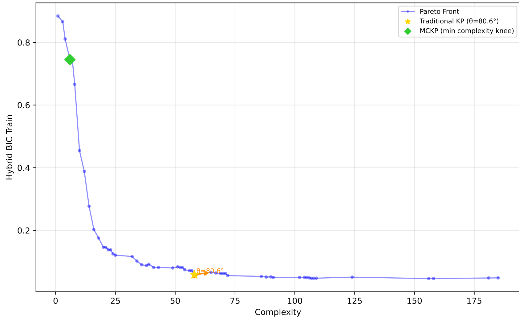
227_cpu_small - Run 10 - SVP - Hybrid BIC Train \lambda_1=0.00, \lambda_2=1.00, \lambda_3=0.00 | Difficulty: 1.00 | Method: hmr
