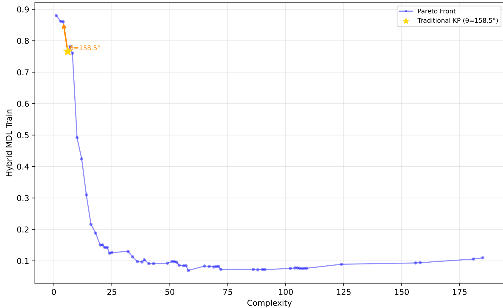
227_cpu_small - Run 10 - SVP - Hybrid MDL Train \lambda_1=0.00, \lambda_2=0.80, \lambda_3=0.30 | Difficulty: 1.00 | Method: hmr
