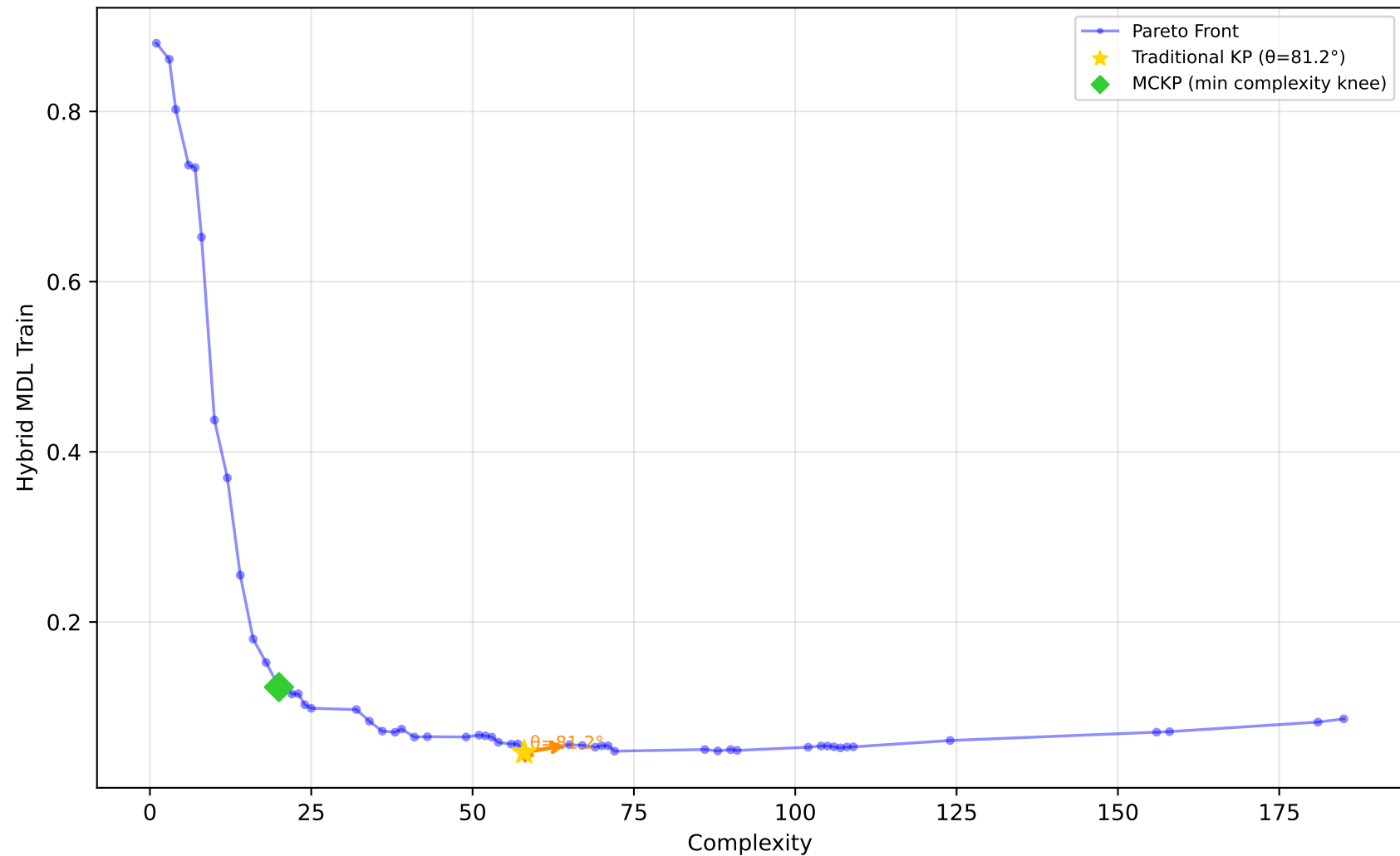
227_cpu_small - Run 10 - SVP - Hybrid MDL Train \lambda_1=0.00, \lambda_2=1.00, \lambda_3=0.00 | Difficulty: 1.00 | Method: hmr
