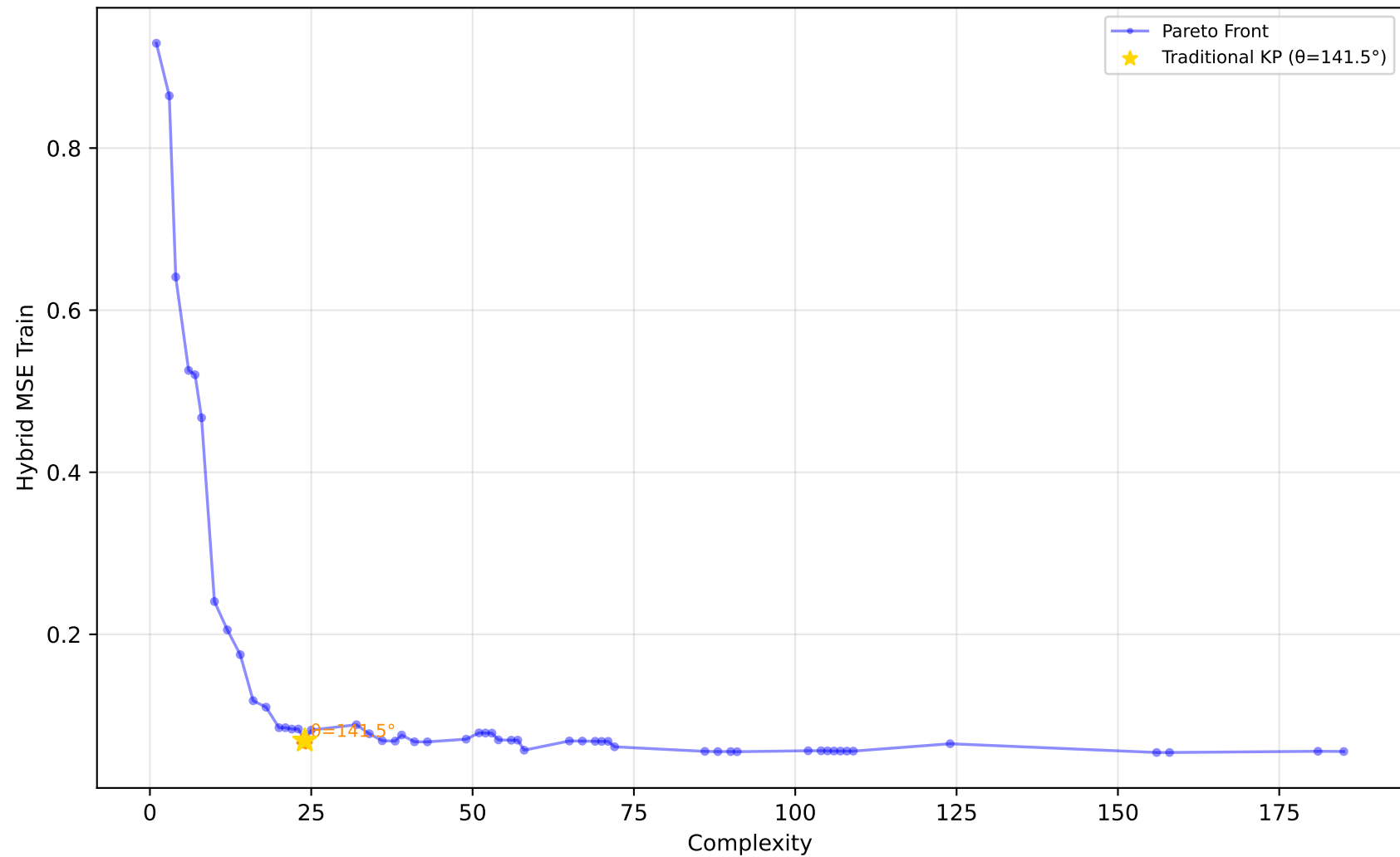
227_cpu_small - Run 10 - SVP - Hybrid MSE Train \lambda_1=0.00, \lambda_2=0.80, \lambda_3=0.30 | Difficulty: 1.00 | Method: hmr
