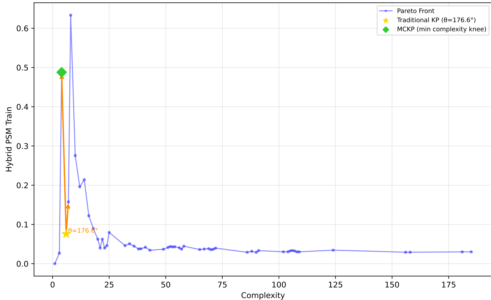
227_cpu_small - Run 10 - SVP - Hybrid PSM Train \lambda_1=0.00, \lambda_2=1.00, \lambda_3=0.00 | Difficulty: 1.00 | Method: hmr
