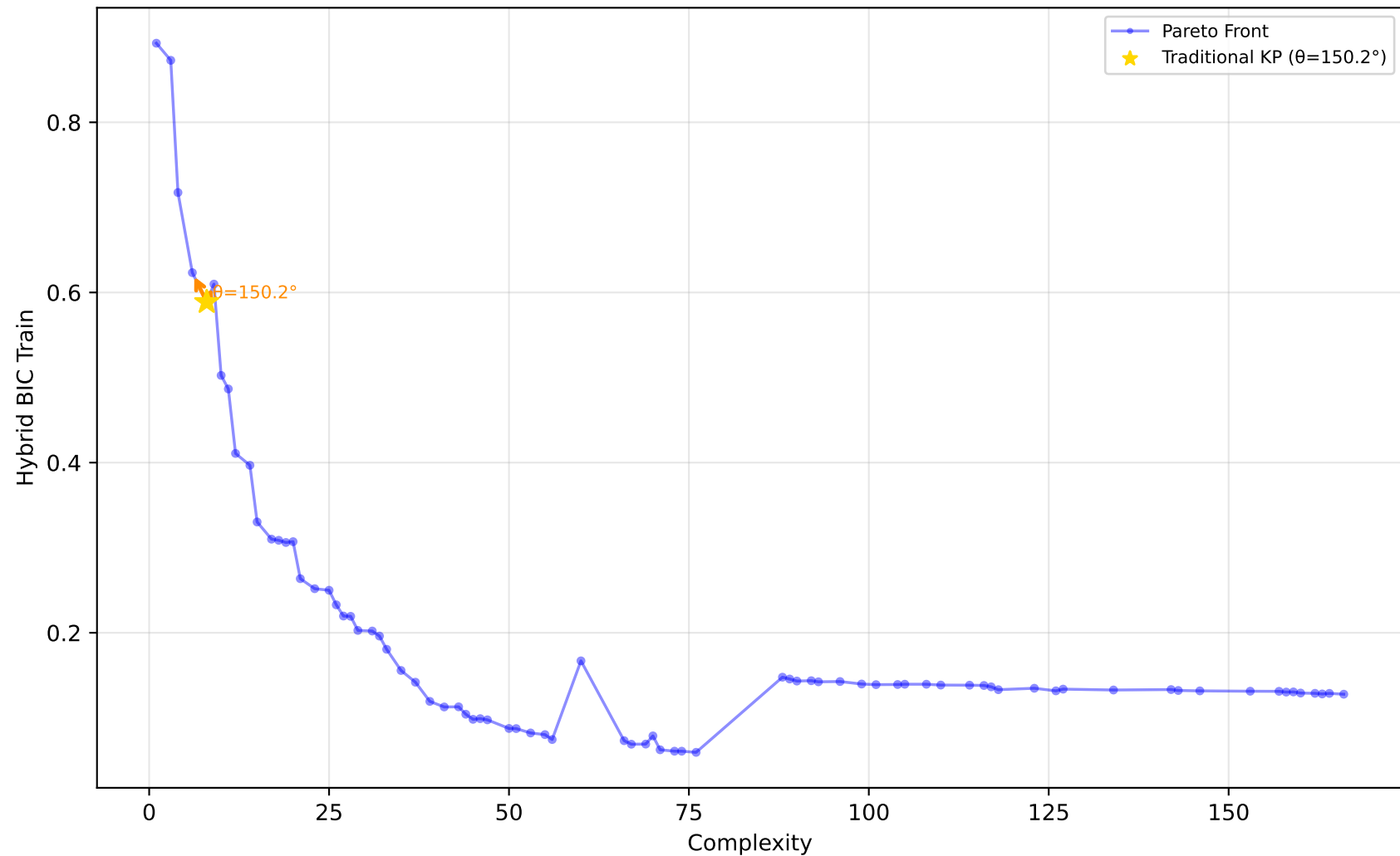
227_cpu_small - Run 11 - MVP - Hybrid BIC Train \lambda_1=0.00, \lambda_2=0.90, \lambda_3=0.10 | Difficulty: 1.00 | Method: hmr
