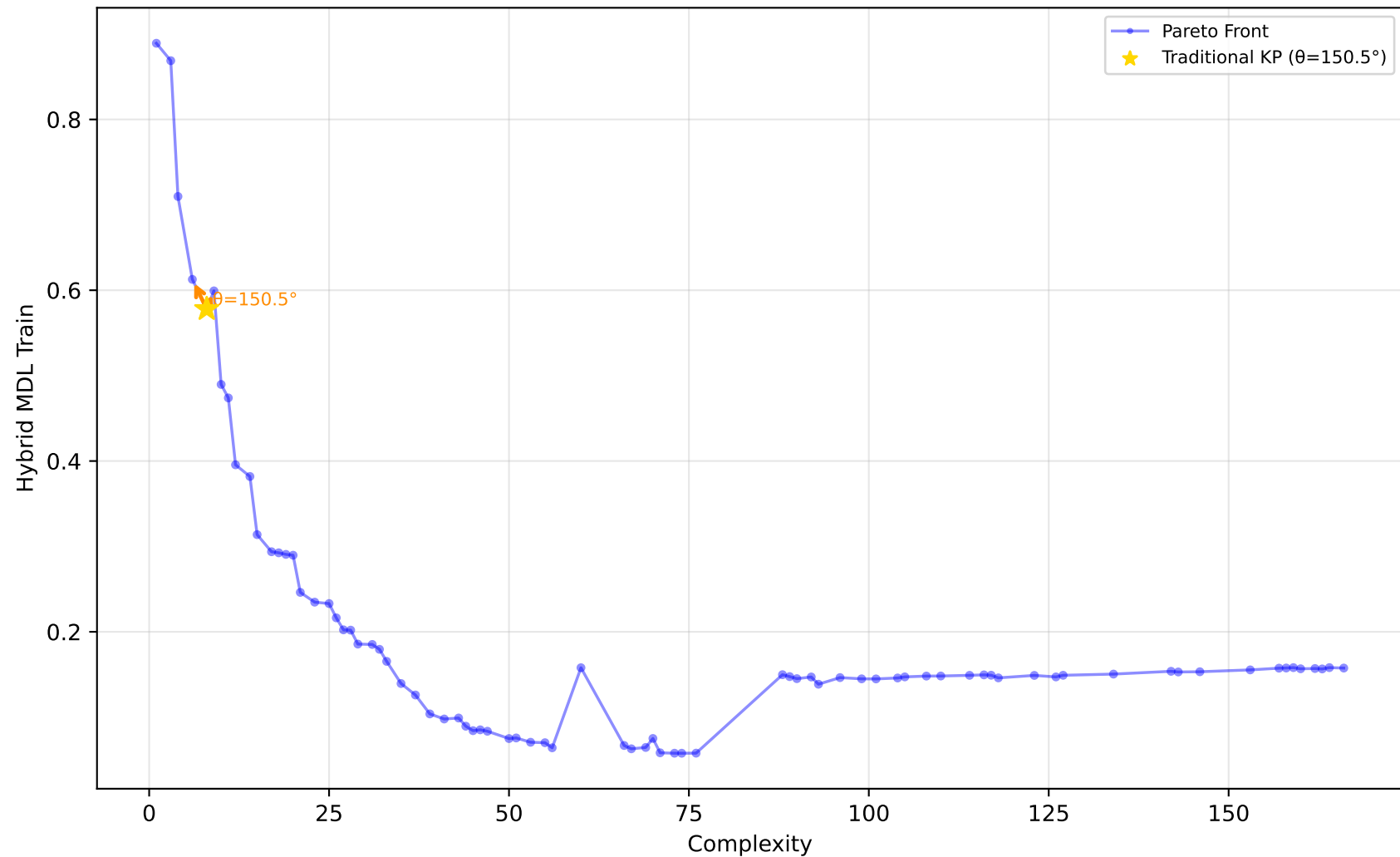
227_cpu_small - Run 11 - MVP - Hybrid MDL Train \lambda_1=0.00, \lambda_2=0.90, \lambda_3=0.10 | Difficulty: 1.00 | Method: hmr
