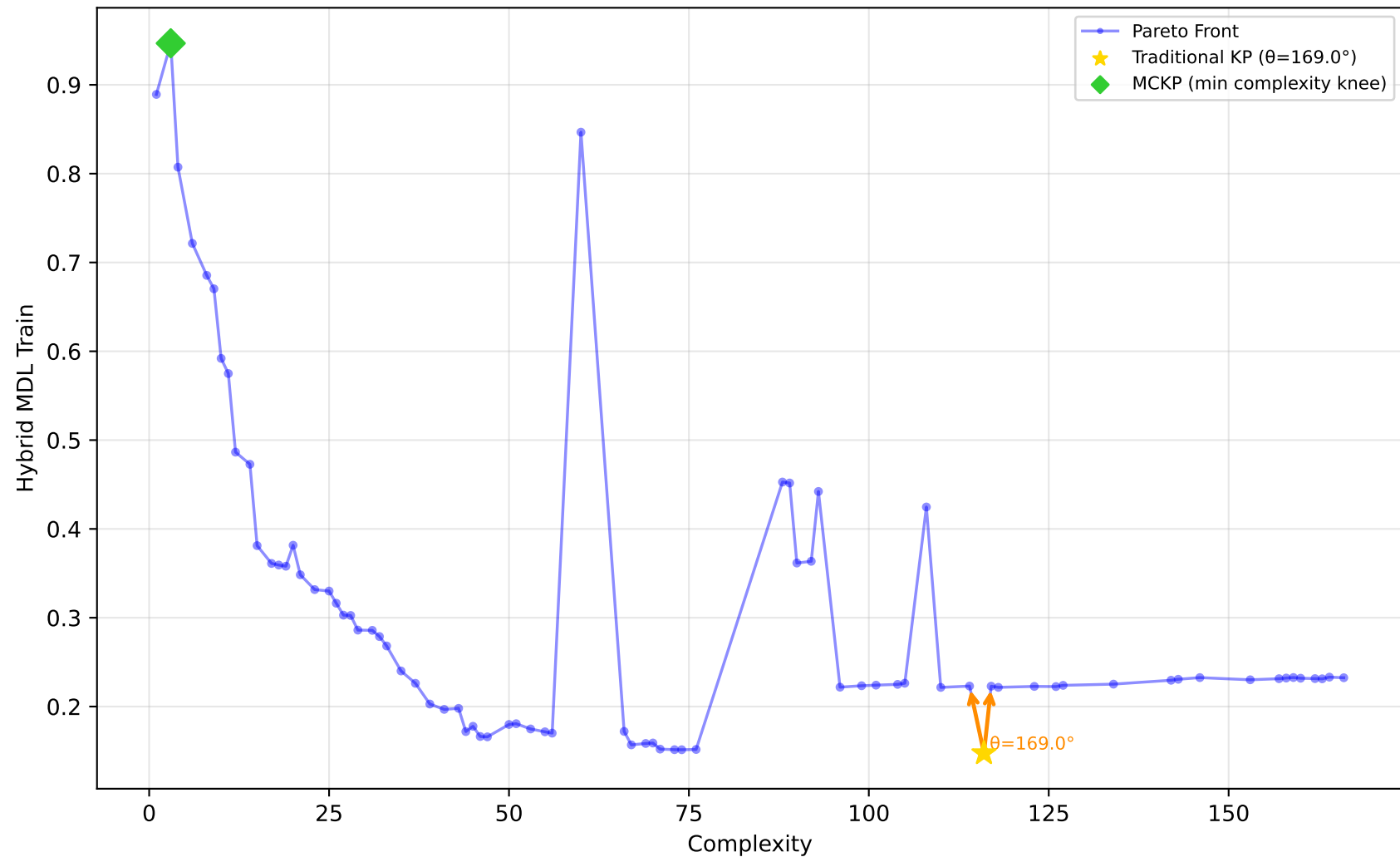
227_cpu_small - Run 11 - MVP - Hybrid MDL Train \lambda_1=0.80, \lambda_2=0.20, \lambda_3=0.00 | Difficulty: 1.00 | Method: hmr
