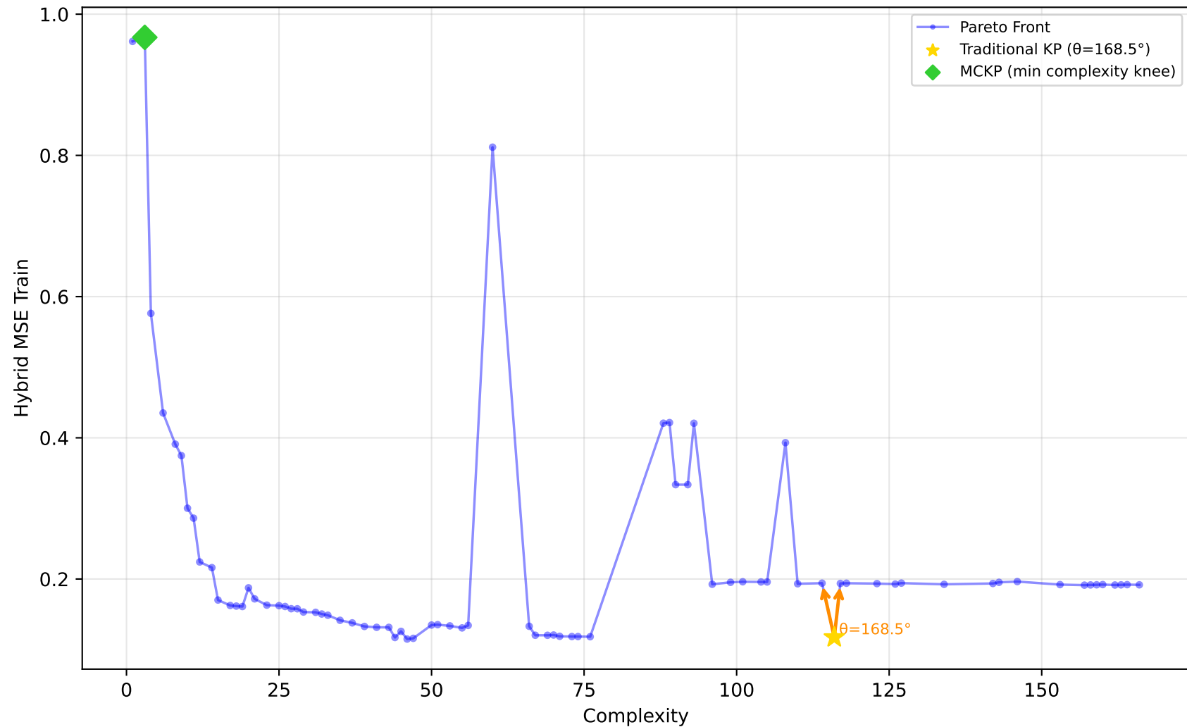
227_cpu_small - Run 11 - MVP - Hybrid MSE Train \lambda_1=0.80, \lambda_2=0.20, \lambda_3=0.00 | Difficulty: 1.00 | Method: hmr
