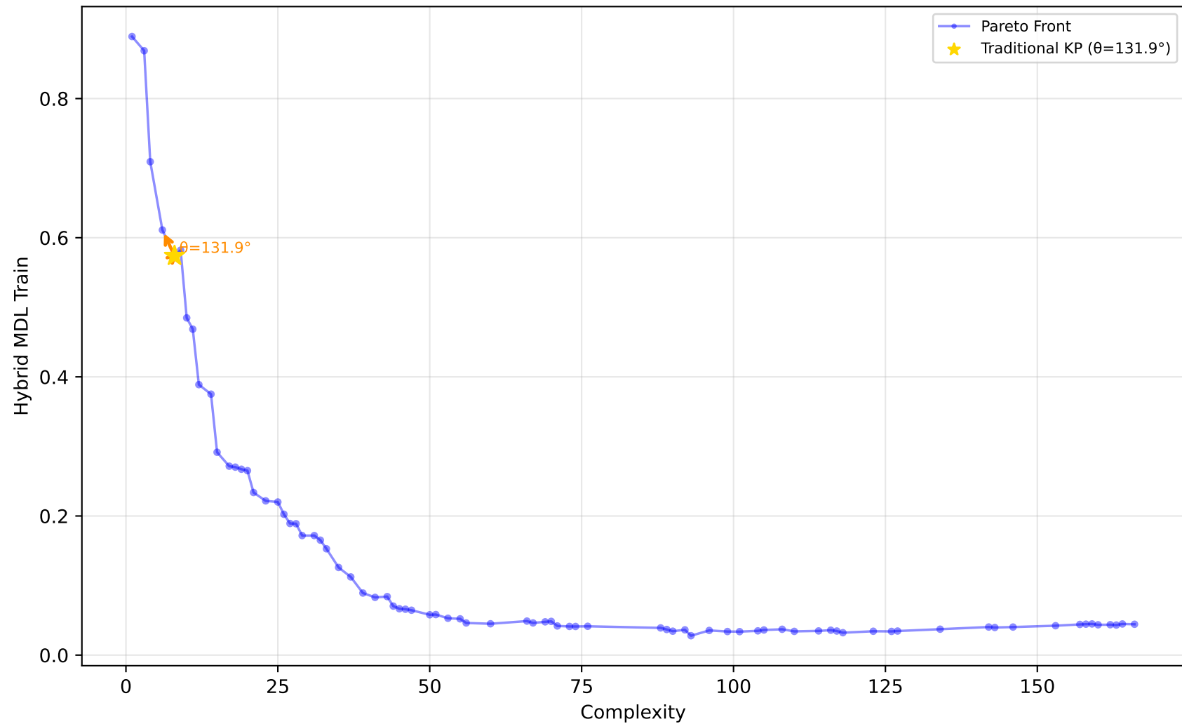
227_cpu_small - Run 11 - SVP - Hybrid MDL Train \lambda_1=0.00, \lambda_2=1.00, \lambda_3=0.00 | Difficulty: 1.00 | Method: hmr
