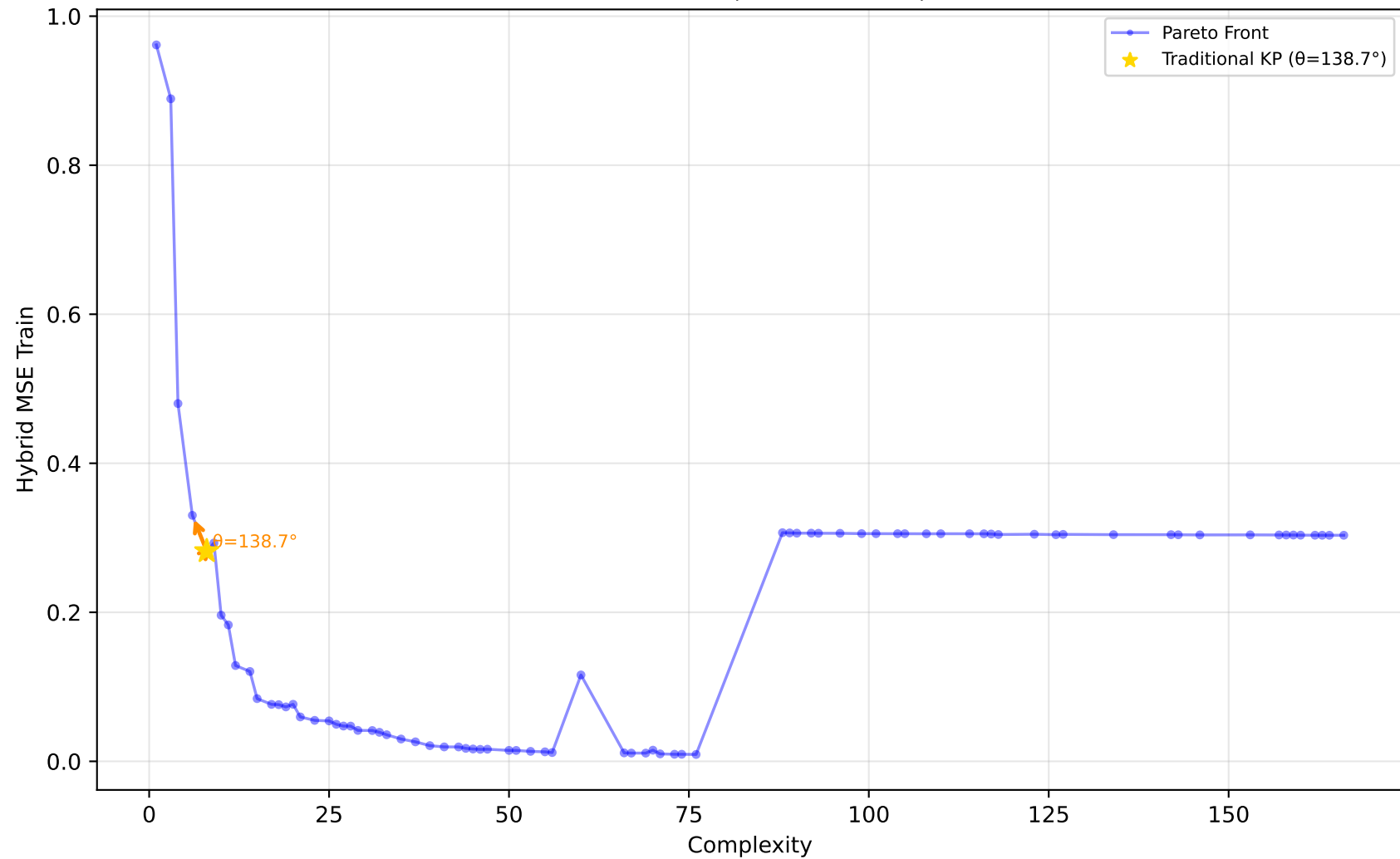
227_cpu_small - Run 11 - SVP - Hybrid MSE Train \lambda_1=0.00, \bar{\lambda}_2=0.80, \lambda_3=0.30 | Difficulty: 1.00 | Method: hmr
