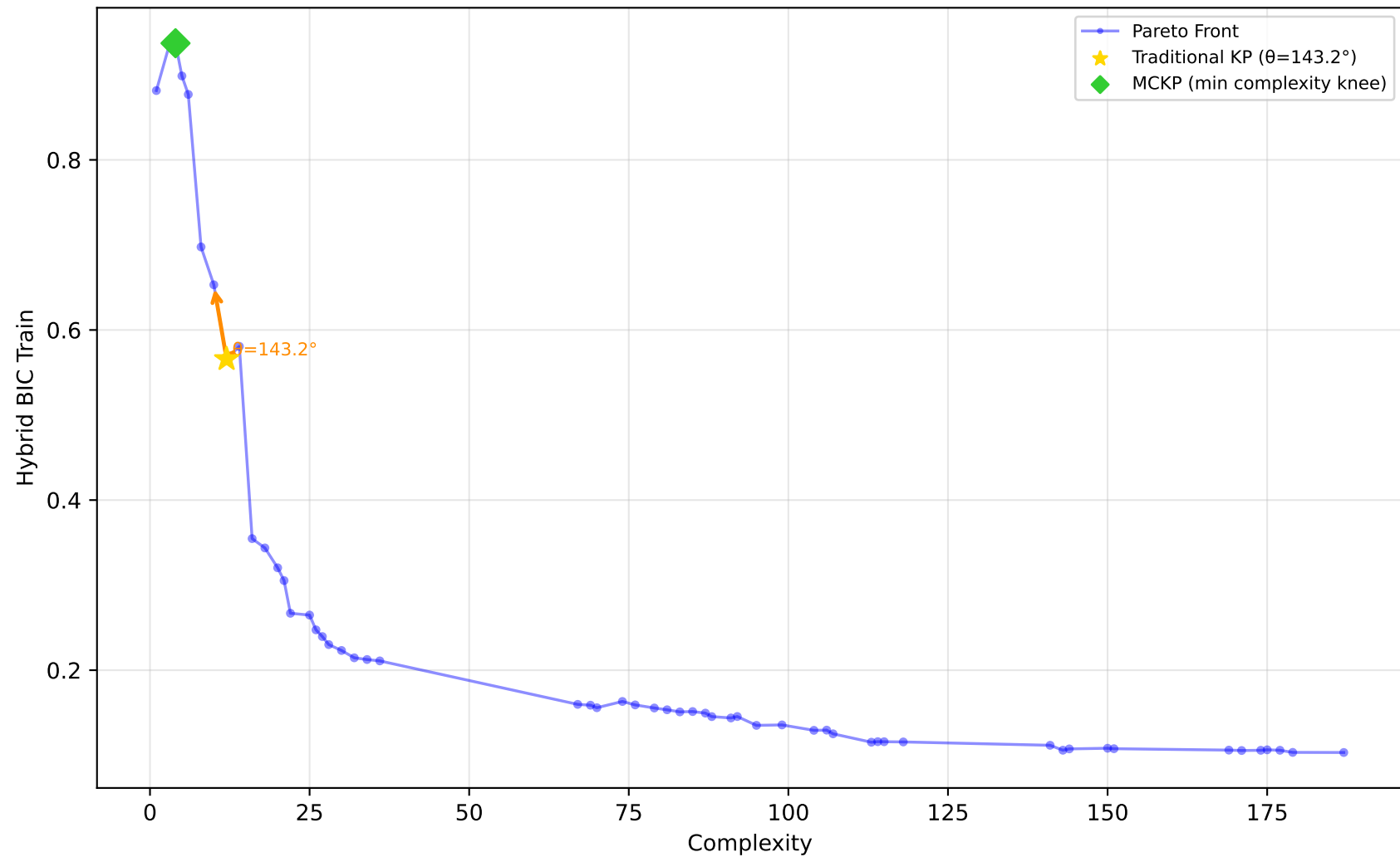
227_cpu_small - Run 12 - MVP - Hybrid BIC Train \lambda_1=0.80, \bar{\lambda}_2=0.20, \lambda_3=0.00 | Difficulty: 1.00 | Method: hmr
