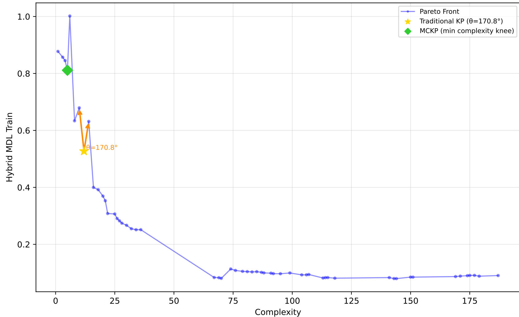
227_cpu_small - Run 12 - MVP - Hybrid MDL Train \lambda_1=0.00, \lambda_2=0.90, \lambda_3=0.10 | Difficulty: 1.00 | Method: hmr
