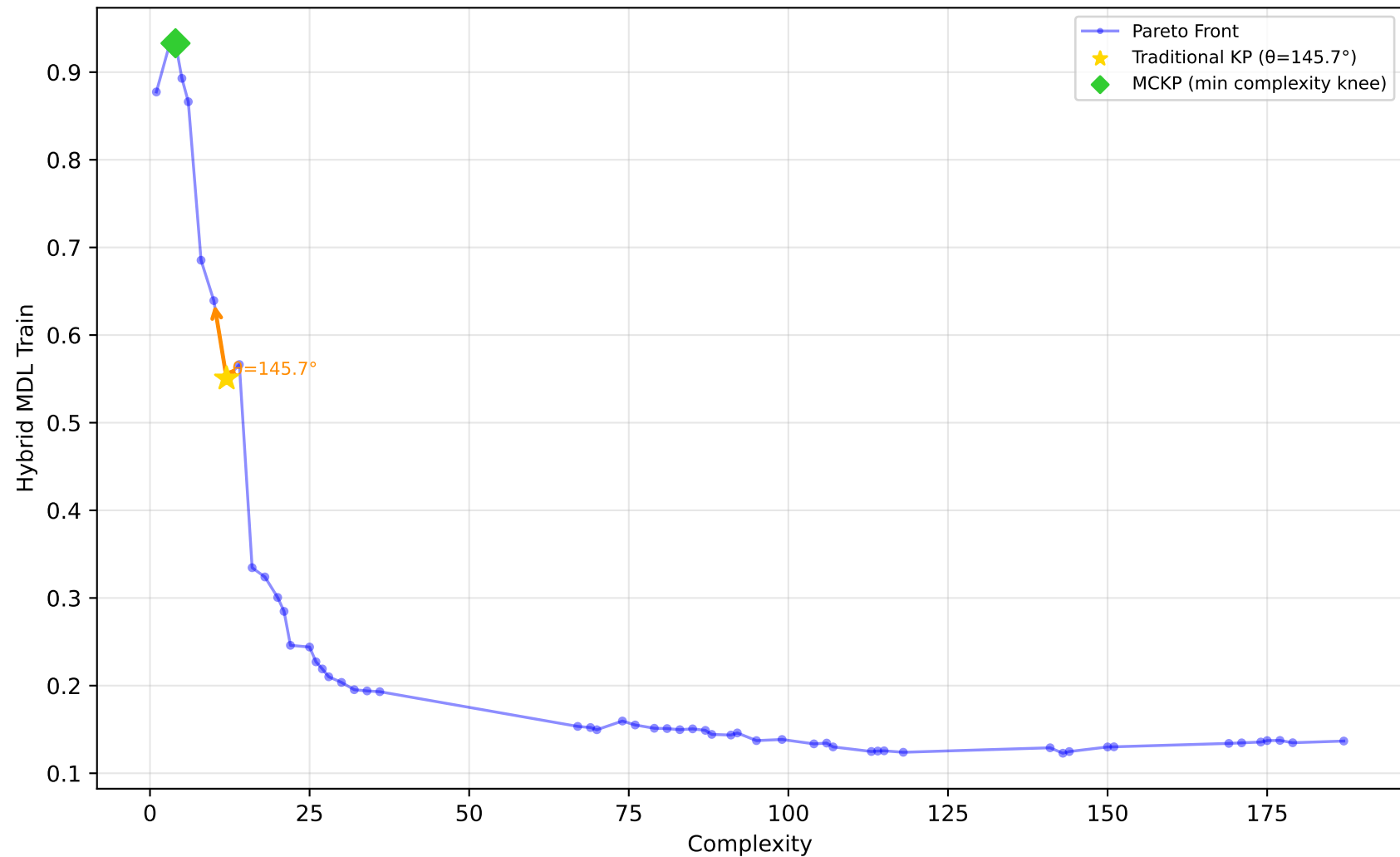
227_cpu_small - Run 12 - MVP - Hybrid MDL Train \lambda_1=0.80, \lambda_2=0.20, \lambda_3=0.00 | Difficulty: 1.00 | Method: hmr
