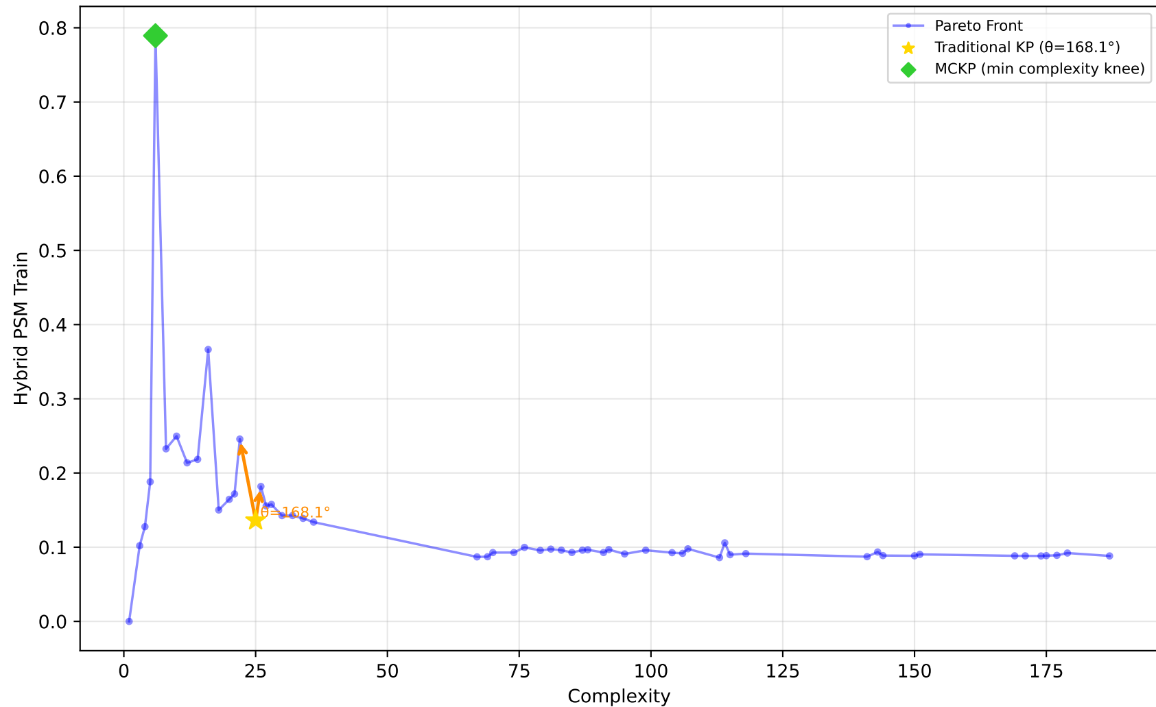
227_cpu_small - Run 12 - MVP - Hybrid PSM Train \lambda_1=0.80, \lambda_2=0.20, \lambda_3=0.00 | Difficulty: 1.00 | Method: hmr
