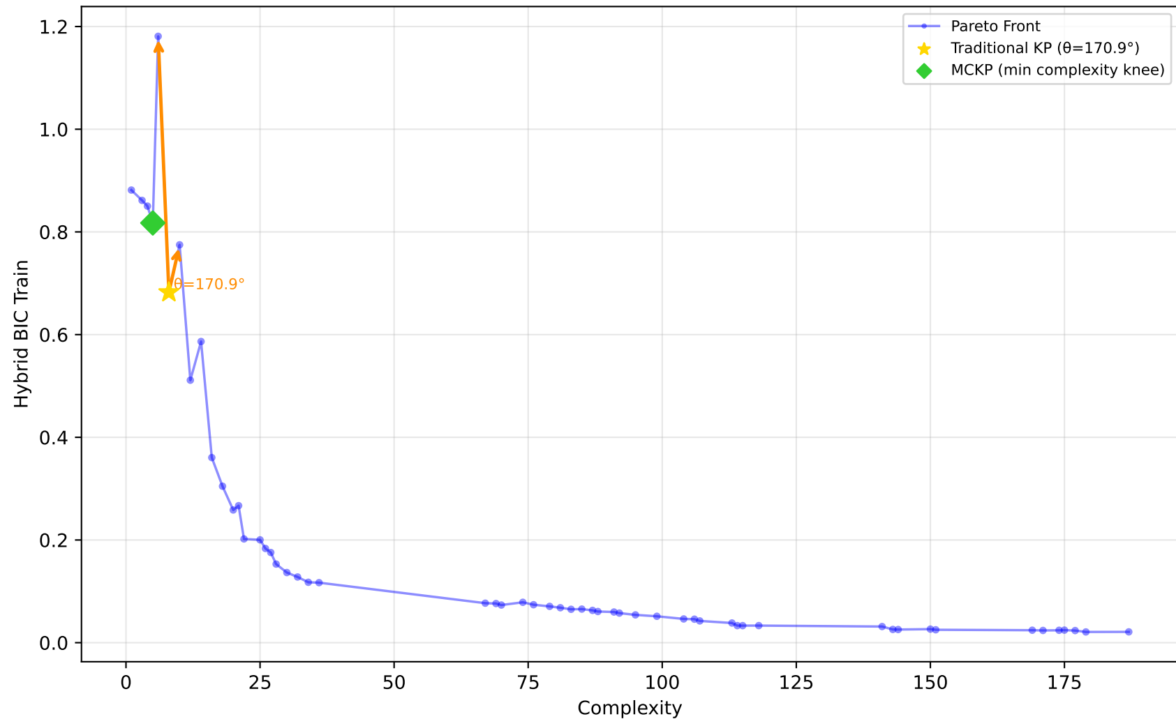
227_cpu_small - Run 12 - SVP - Hybrid BIC Train \lambda_1=0.00, \bar{\lambda}_2=0.80, \lambda_3=0.30 | Difficulty: 1.00 | Method: hmr
