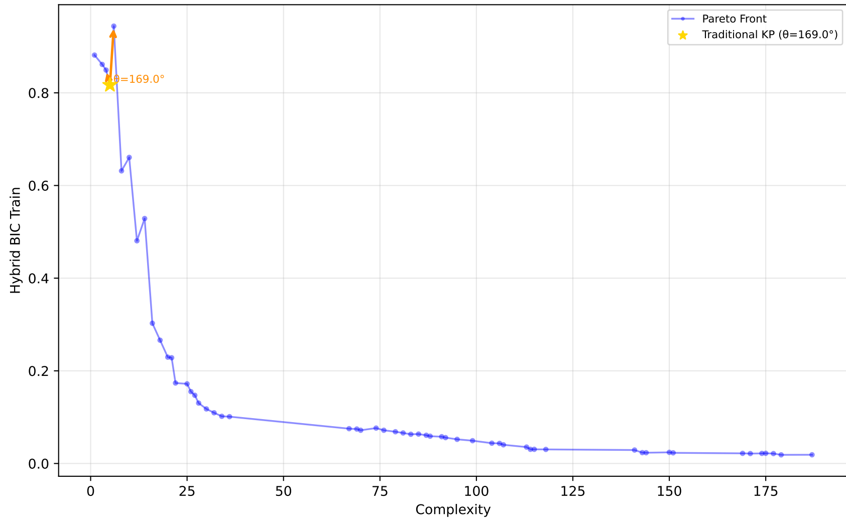
227_cpu_small - Run 12 - SVP - Hybrid BIC Train \lambda_1=0.00, \lambda_2=1.00, \lambda_3=0.00 | Difficulty: 1.00 | Method: hmr
