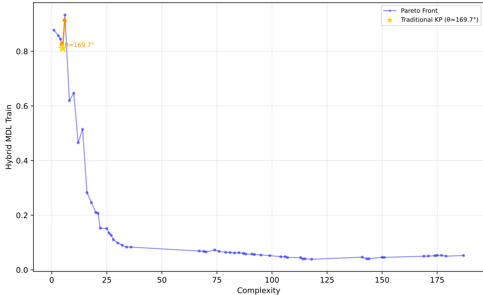
227_cpu_small - Run 12 - SVP - Hybrid MDL Train \lambda_1=0.00, \lambda_2=1.00, \lambda_3=0.00 | Difficulty: 1.00 | Method: hmr
