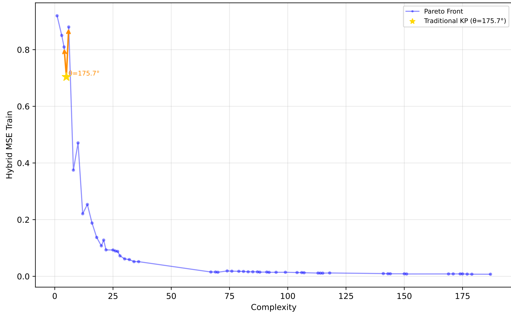
227_cpu_small - Run 12 - SVP - Hybrid MSE Train \lambda_1=0.00, \lambda_2=0.80, \lambda_3=0.30 | Difficulty: 1.00 | Method: hmr
