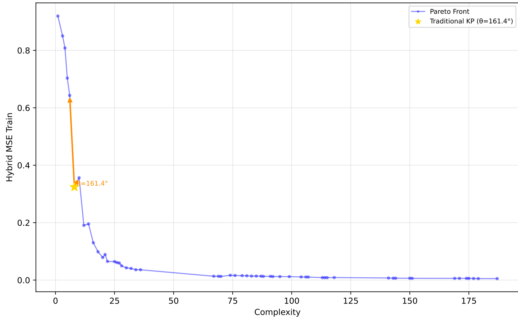
227_cpu_small - Run 12 - SVP - Hybrid MSE Train \lambda_1=0.00, \lambda_2=1.00, \lambda_3=0.00 | Difficulty: 1.00 | Method: hmr
