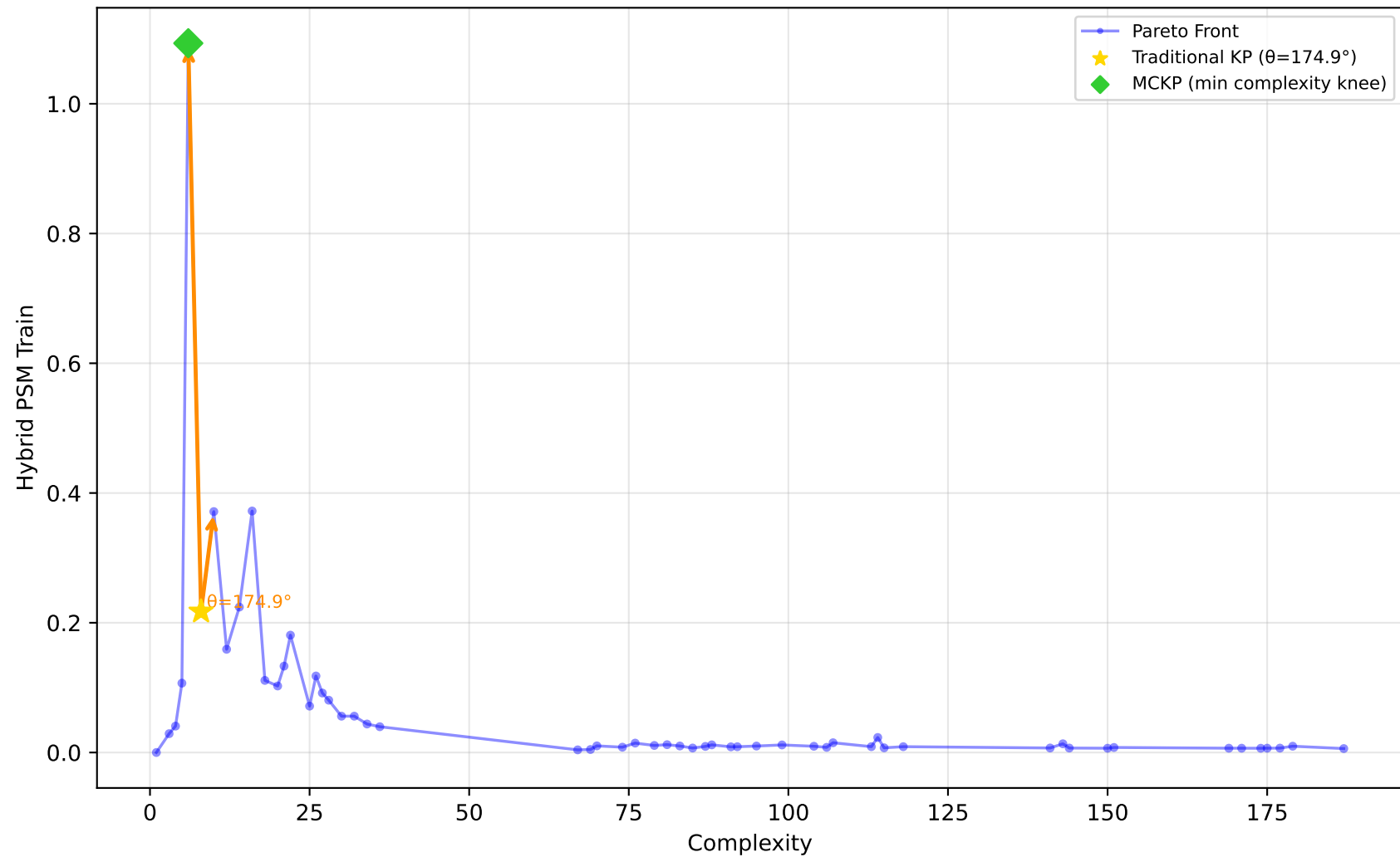
227_cpu_small - Run 12 - SVP - Hybrid PSM Train \lambda_1=0.00, \lambda_2=0.80, \lambda_3=0.30 | Difficulty: 1.00 | Method: hmr
