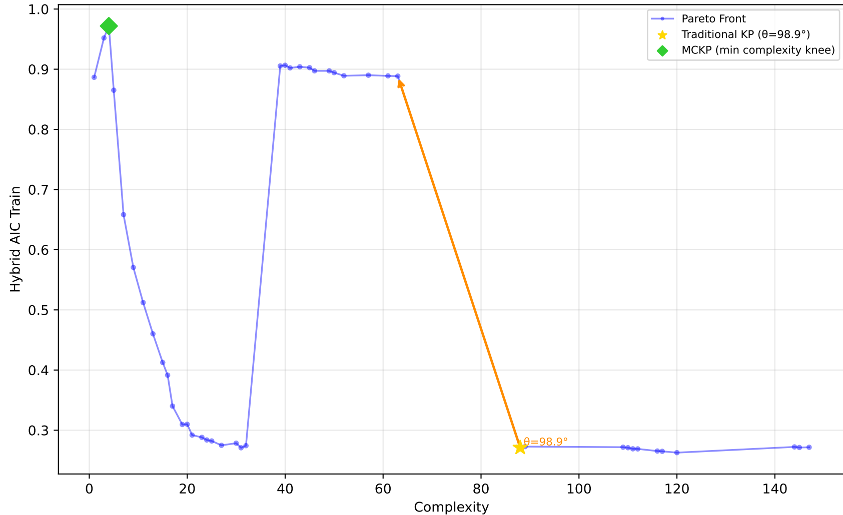
227_cpu_small - Run 13 - MVP - Hybrid AIC Train \lambda_1=0.80, \lambda_2=0.20, \lambda_3=0.00 | Difficulty: 1.00 | Method: hmr
