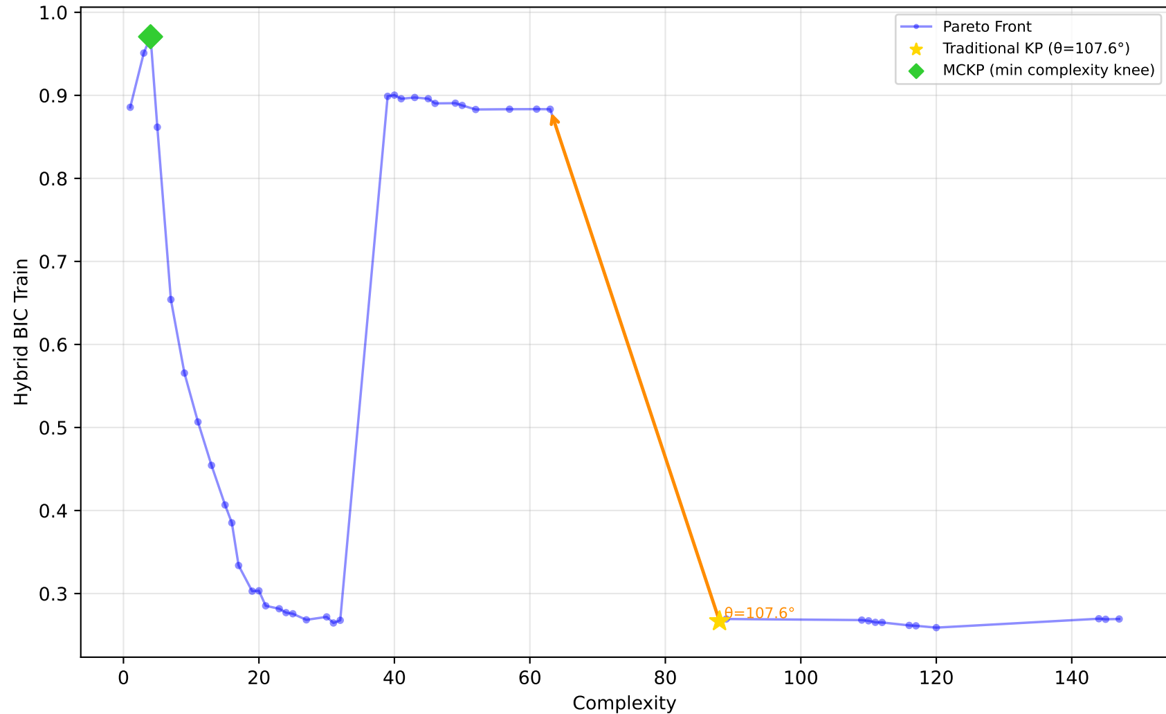
227_cpu_small - Run 13 - MVP - Hybrid BIC Train \lambda_1=0.80, \bar{\lambda}_2=0.20, \lambda_3=0.00 | Difficulty: 1.00 | Method: hmr
