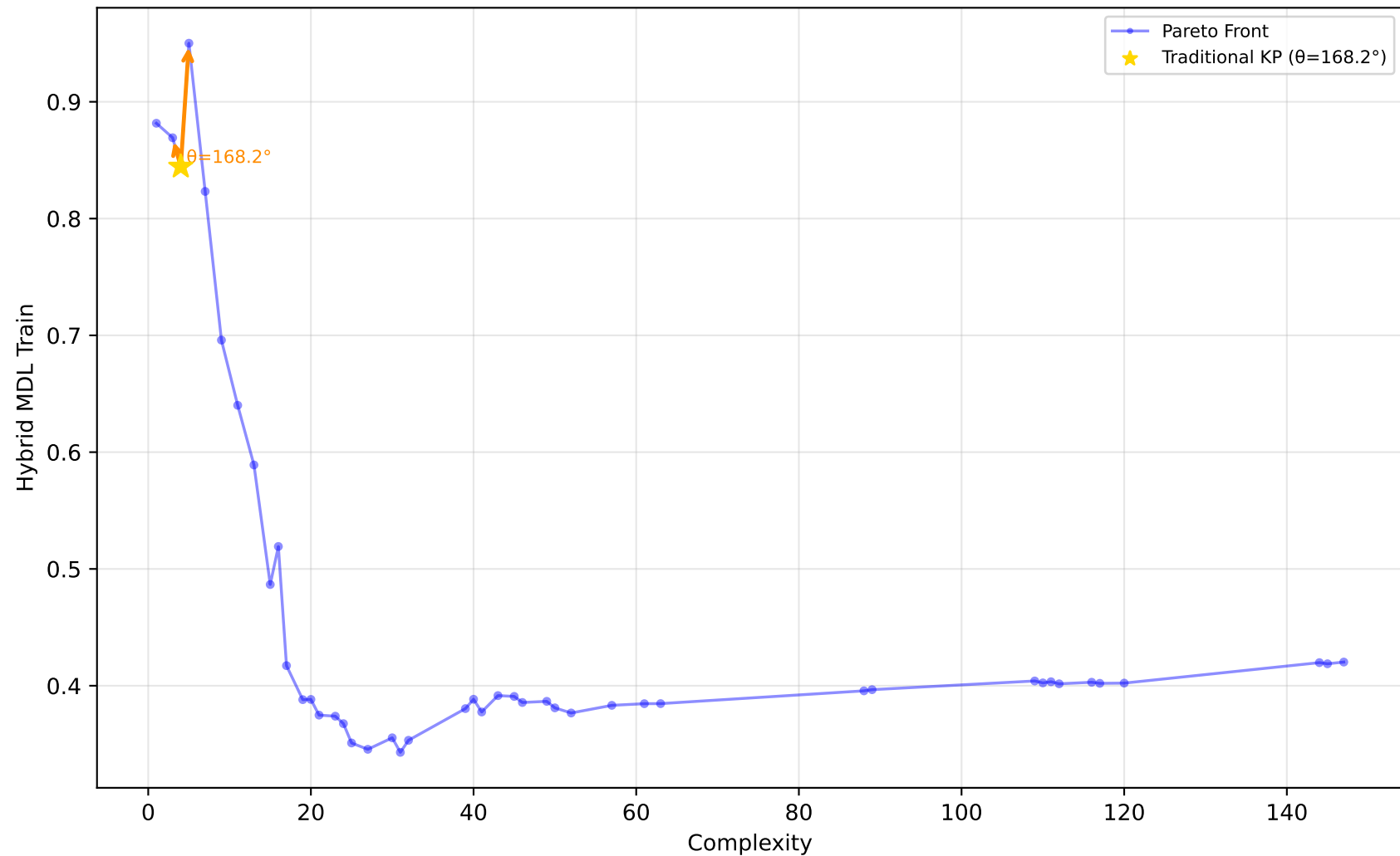
227_cpu_small - Run 13 - MVP - Hybrid MDL Train \lambda_1=0.00, \lambda_2=0.90, \lambda_3=0.10 | Difficulty: 1.00 | Method: hmr
