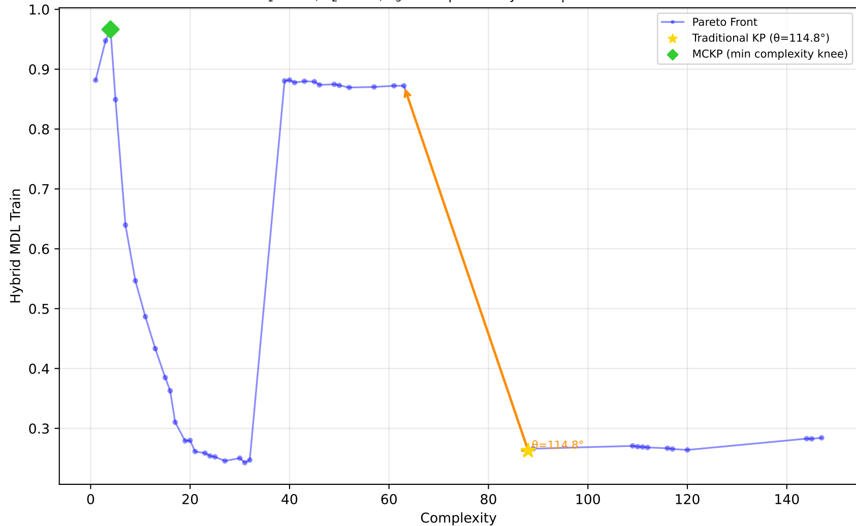
227_cpu_small - Run 13 - MVP - Hybrid MDL Train \lambda_1=0.80, \lambda_2=0.20, \lambda_3=0.00 | Difficulty: 1.00 | Method: hmr
