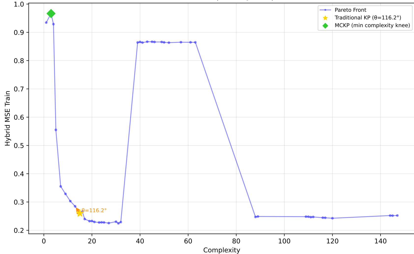
227_cpu_small - Run 13 - MVP - Hybrid MSE Train \lambda_1=0.80, \lambda_2=0.20, \lambda_3=0.00 | Difficulty: 1.00 | Method: hmr
