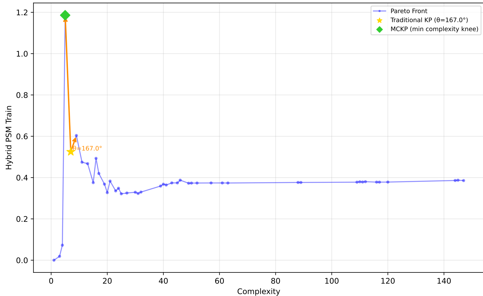
227_cpu_small - Run 13 - MVP - Hybrid PSM Train \lambda_1=0.00, \lambda_2=0.90, \lambda_3=0.10 | Difficulty: 1.00 | Method: hmr
