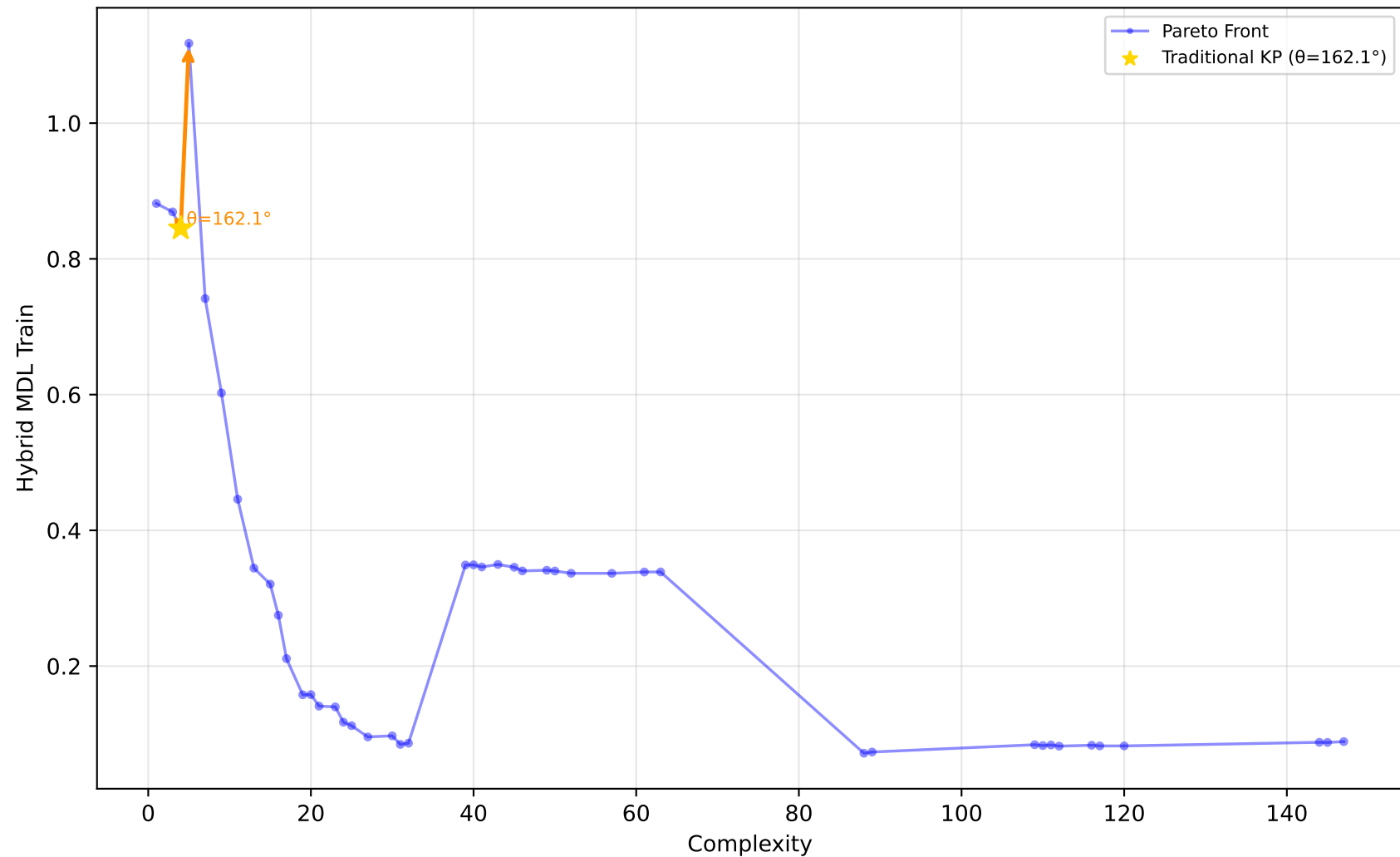
227_cpu_small - Run 13 - SVP - Hybrid MDL Train \lambda_1=0.00, \lambda_2=0.80, \lambda_3=0.30 | Difficulty: 1.00 | Method: hmr
