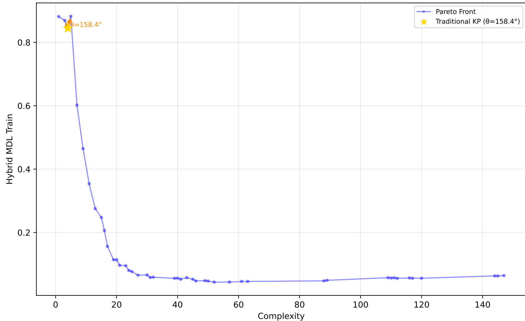
227_cpu_small - Run 13 - SVP - Hybrid MDL Train \lambda_1=0.00, \lambda_2=1.00, \lambda_3=0.00 | Difficulty: 1.00 | Method: hmr
