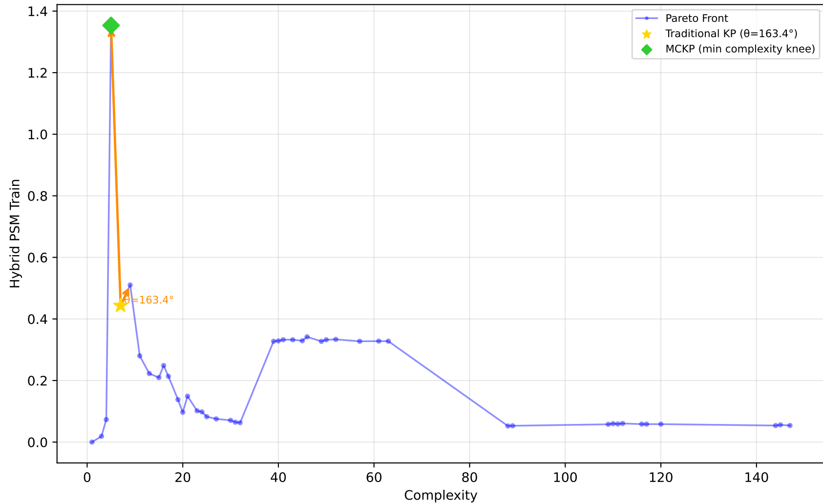
227_cpu_small - Run 13 - SVP - Hybrid PSM Train \lambda_1=0.00, \lambda_2=0.80, \lambda_3=0.30 | Difficulty: 1.00 | Method: hmr
