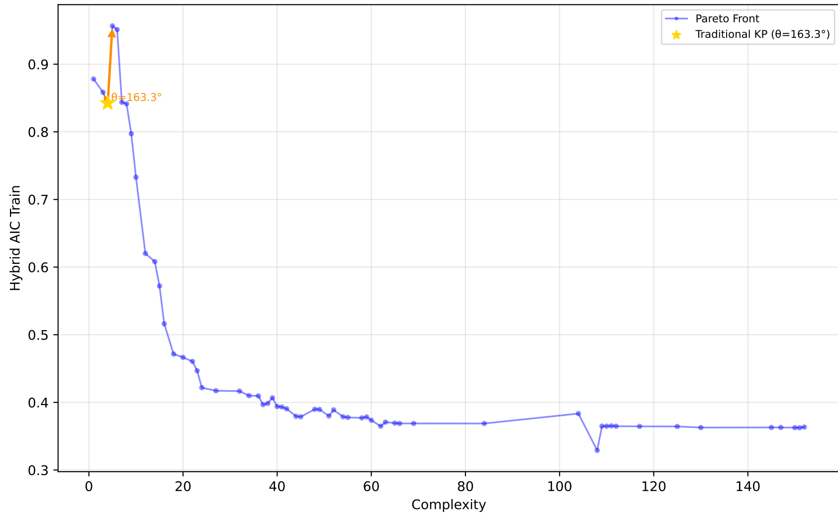
227_cpu_small - Run 14 - MVP - Hybrid AIC Train \lambda_1=0.00, \lambda_2=0.90, \lambda_3=0.10 | Difficulty: 1.00 | Method: hmr
