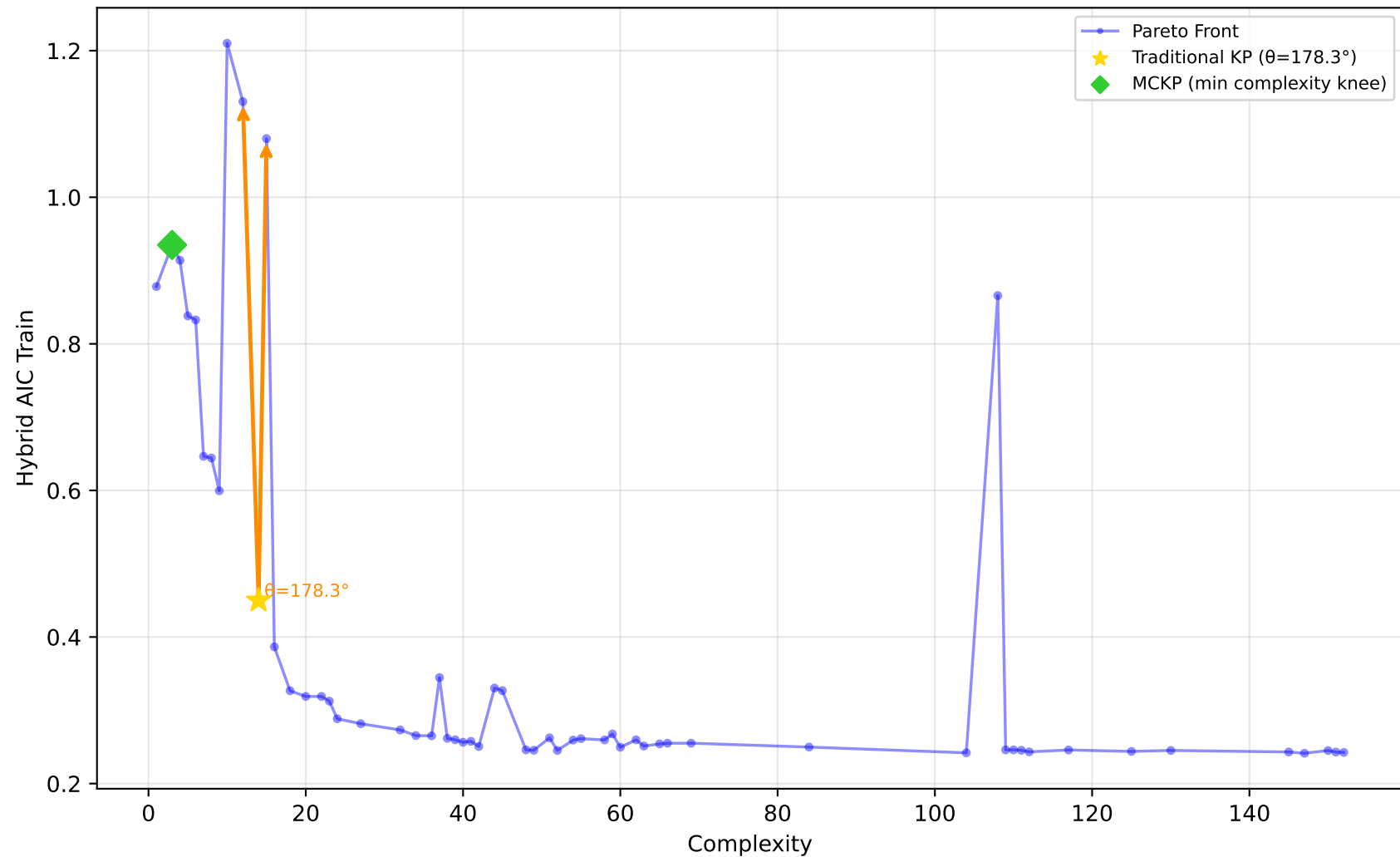
227_cpu_small - Run 14 - MVP - Hybrid AIC Train \lambda_1=0.80, \bar{\lambda}_2=0.20, \lambda_3=0.00 | Difficulty: 1.00 | Method: hmr
