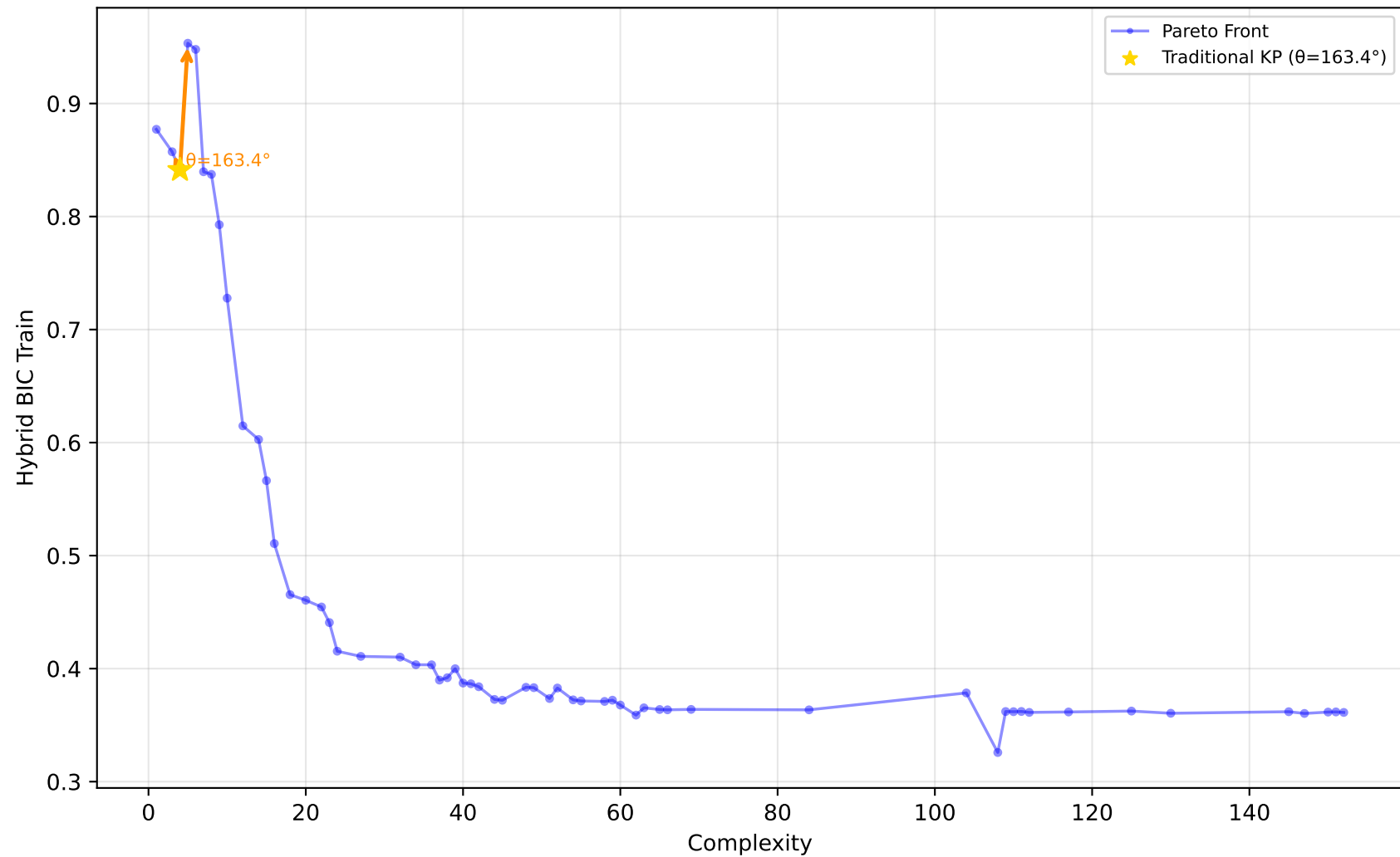
227_cpu_small - Run 14 - MVP - Hybrid BIC Train \lambda_1=0.00, \lambda_2=0.90, \lambda_3=0.10 | Difficulty: 1.00 | Method: hmr
