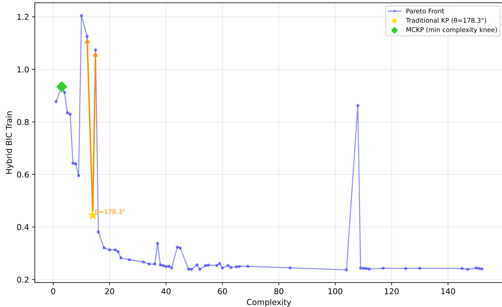
227_cpu_small - Run 14 - MVP - Hybrid BIC Train \lambda_1=0.80, \bar{\lambda}_2=0.20, \lambda_3=0.00 | Difficulty: 1.00 | Method: hmr
