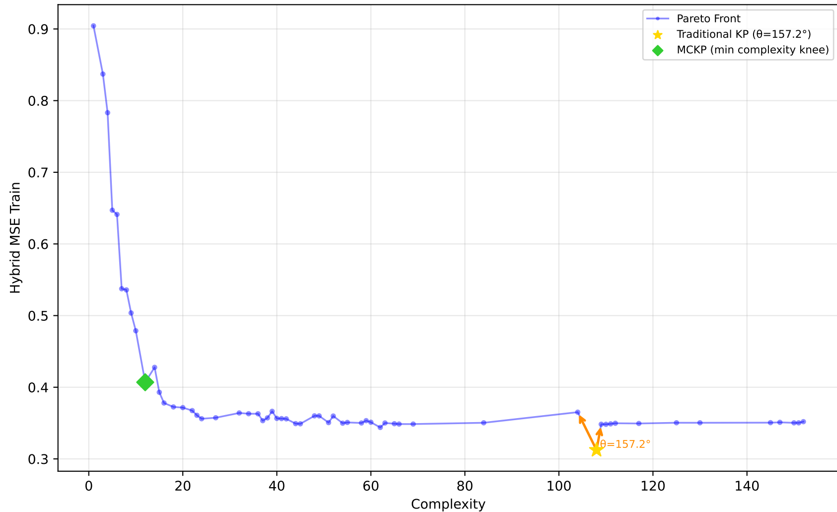
227_cpu_small - Run 14 - MVP - Hybrid MSE Train \lambda_1=0.00, \lambda_2=0.90, \lambda_3=0.10 | Difficulty: 1.00 | Method: hmr
