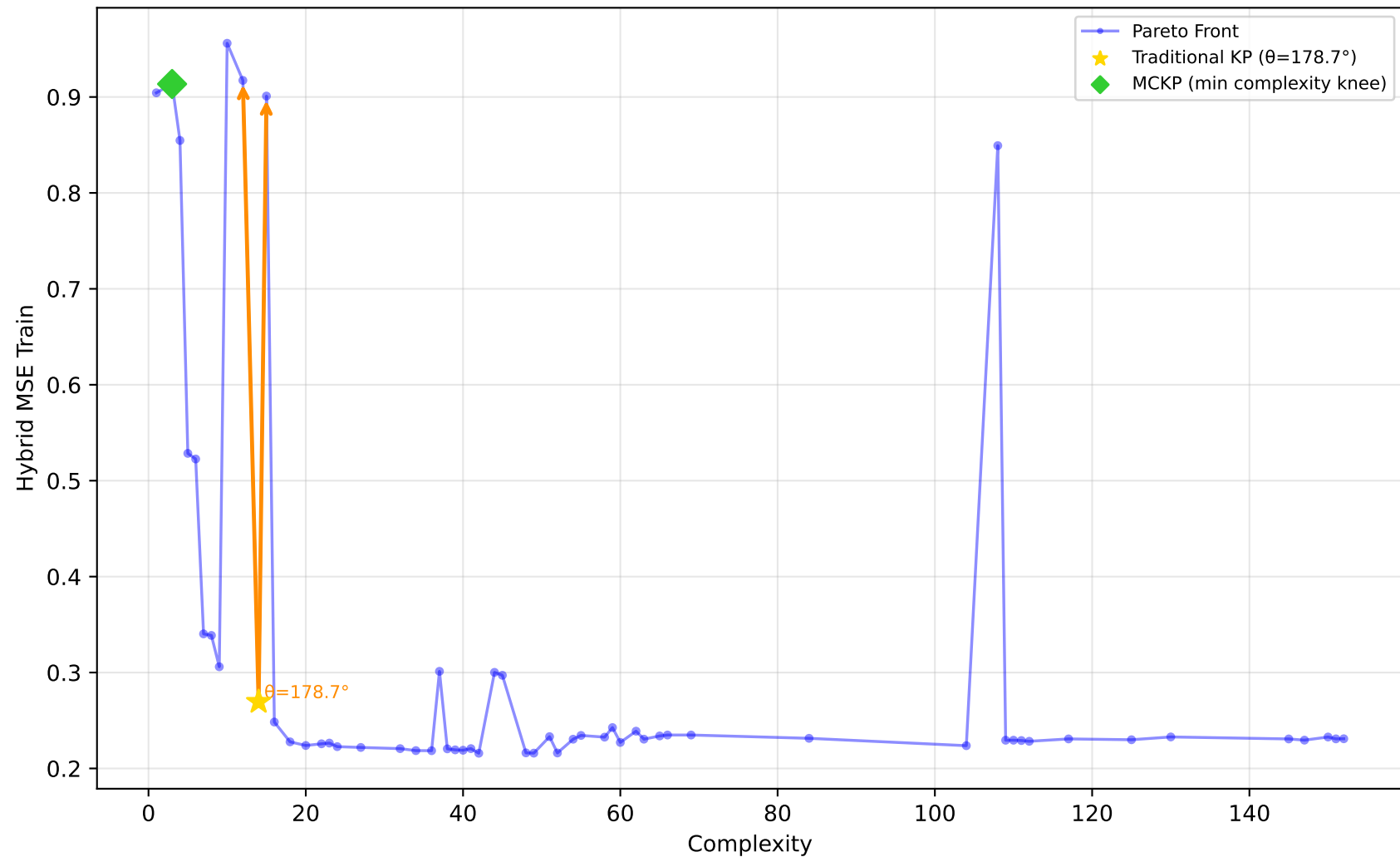
227_cpu_small - Run 14 - MVP - Hybrid MSE Train \lambda_1=0.80, \lambda_2=0.20, \lambda_3=0.00 | Difficulty: 1.00 | Method: hmr
