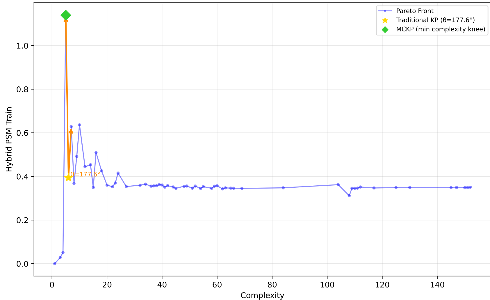
227_cpu_small - Run 14 - MVP - Hybrid PSM Train \lambda_1=0.00, \lambda_2=0.90, \lambda_3=0.10 | Difficulty: 1.00 | Method: hmr
