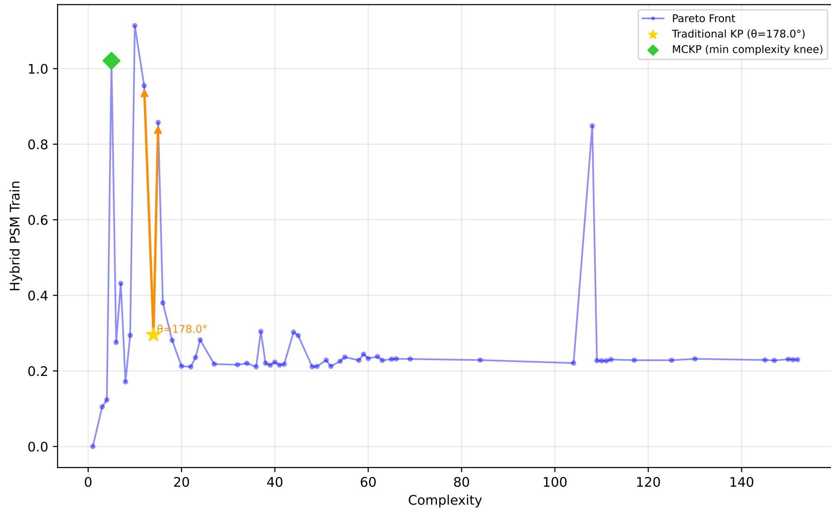
227_cpu_small - Run 14 - MVP - Hybrid PSM Train \lambda_1=0.80, \lambda_2=0.20, \lambda_3=0.00 | Difficulty: 1.00 | Method: hmr
