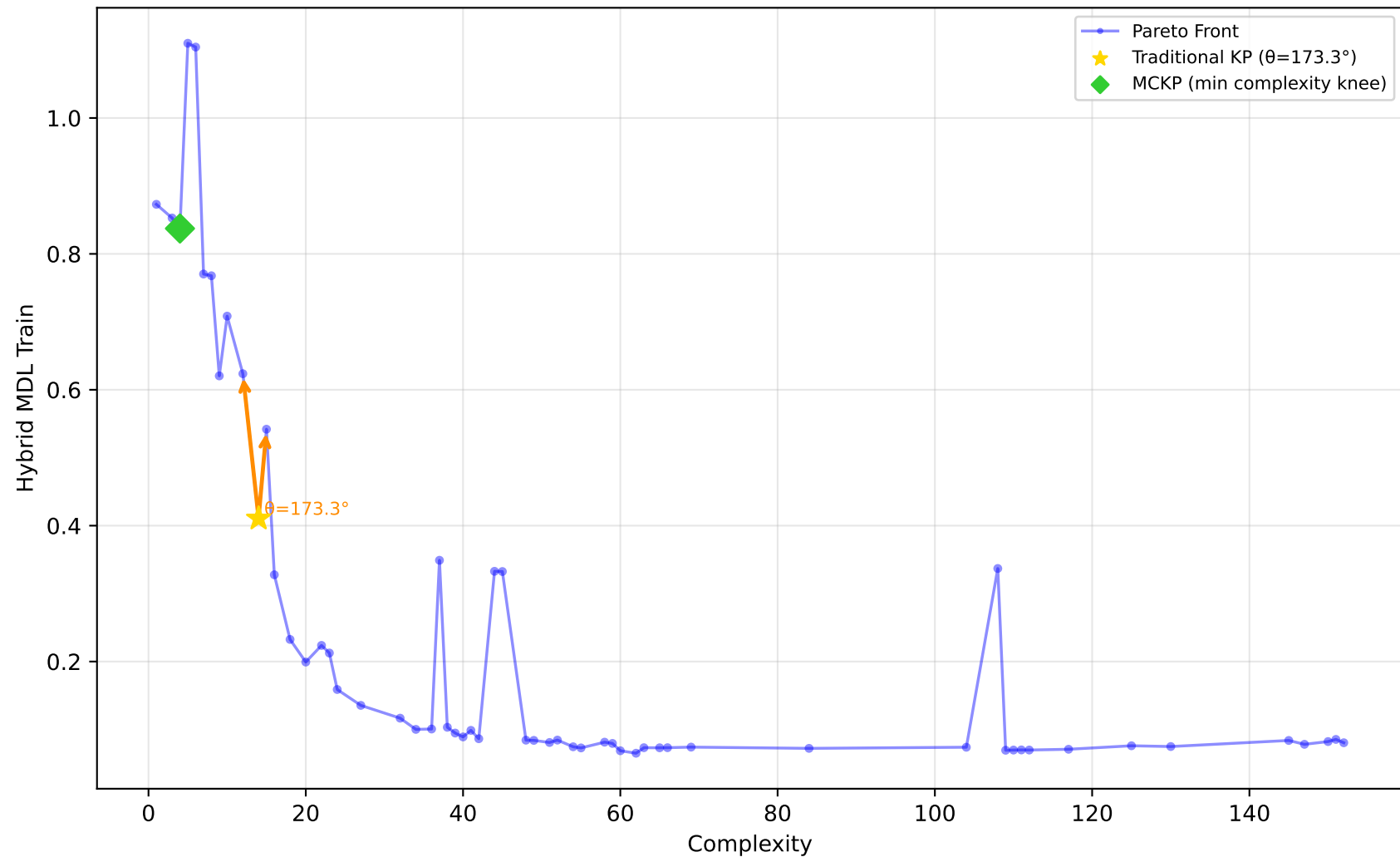
227_cpu_small - Run 14 - SVP - Hybrid MDL Train \lambda_1=0.00, \lambda_2=0.80, \lambda_3=0.30 | Difficulty: 1.00 | Method: hmr
