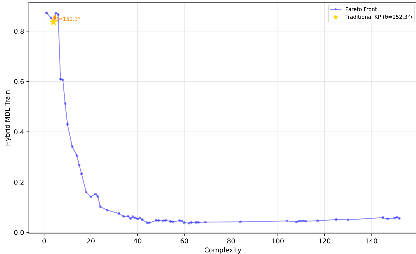
227_cpu_small - Run 14 - SVP - Hybrid MDL Train \lambda_1=0.00, \lambda_2=1.00, \lambda_3=0.00 | Difficulty: 1.00 | Method: hmr
